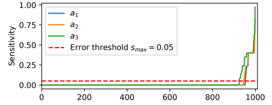
Fig. 1. Results of sensitivity analysis for a 1000 driving scenarios, across three lower fidelity configurations in A_{eval} .
