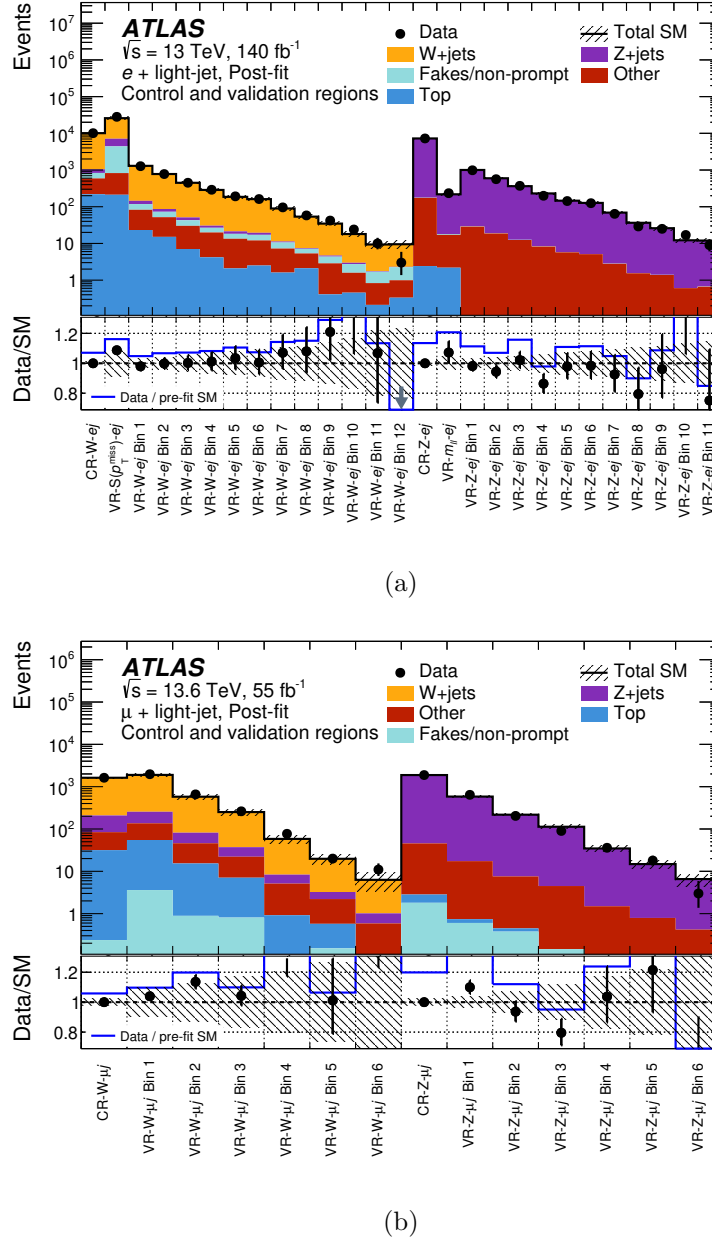
Figure 8. Data (dots) and post-fit SM predictions (histograms) in the VRs for (a) Run 2 of the e + \text{light-jet} and (b) Run 3 of the \mu + \text{light-jet} channels obtained by a CR-only fit. The lower panel shows the ratio of observed data to the total post- and pre-fit SM prediction. Uncertainties in the background estimates include both the statistical and systematic uncertainties, with correlations between uncertainties taken into account. A grey arrow in the lower panel indicates a data point outside the vertical range shown.
