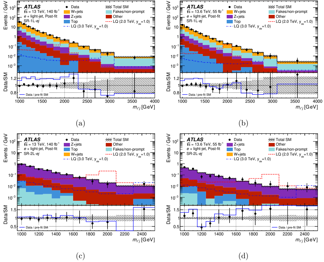
Figure 10. Data (dots) and post-fit SM distribution (histograms) of m_{\ell j} in (a), (b) SR-1L- e j and (c), (d) SR-2L- e j of the e + \text{light-jet} channel obtained by a CR+SR background-only fit for Run 2 and Run 3, respectively. The lower panel shows the ratio of observed data to the total post- and pre-fit SM prediction. The last bin includes the overflow. Uncertainties in the background estimates include both the statistical and systematic uncertainties, with correlations between uncertainties taken into account. The dashed lines show the predicted yields for two benchmark signal models corresponding to \tilde{S}_1(m, y_{de}) = (2.0 \text{ TeV}, 1.0) and \tilde{S}_1(m, y_{de}) = (3.0 \text{ TeV}, 1.0) , respectively.
