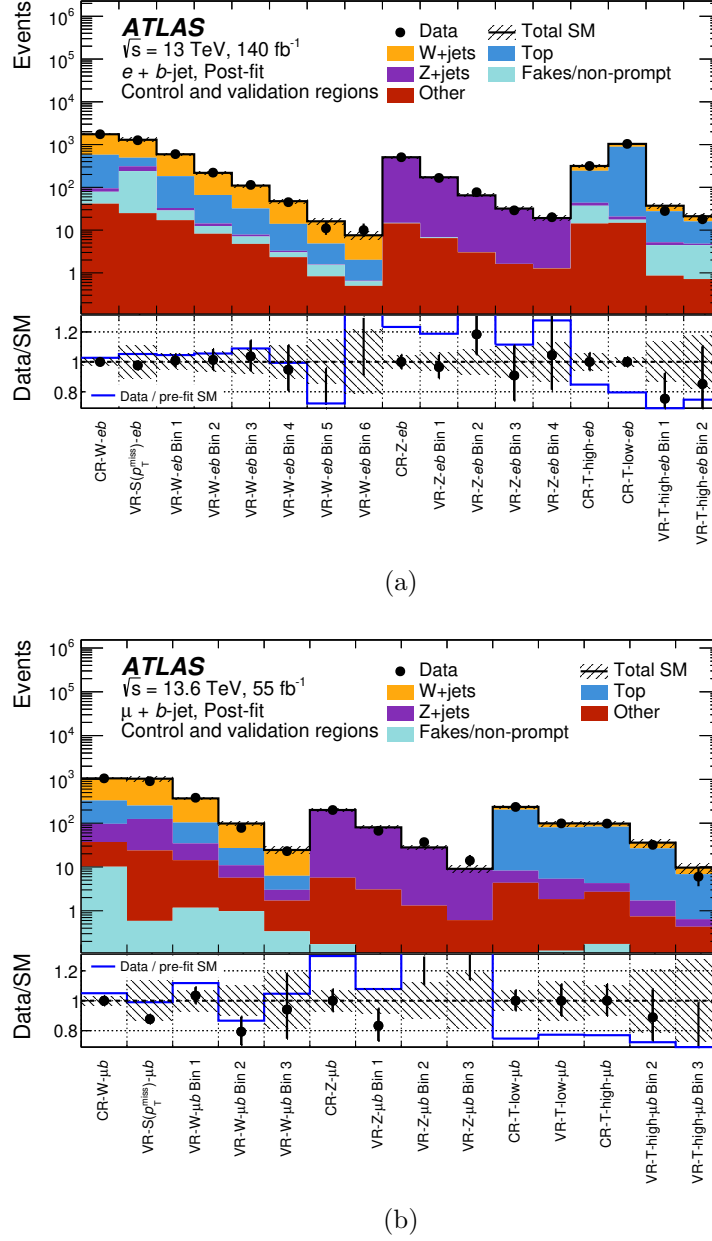
Figure 9. Data (dots) and post-fit SM predictions (histograms) in the VRs for (a) Run 2 of the e+b -jet and (b) Run 3 of the \mu+b -jet channels obtained by a CR-only fit. The lower panel shows the ratio of observed data to the total post- and pre-fit SM prediction. Uncertainties in the background estimates include both the statistical and systematic uncertainties, with correlations between uncertainties taken into account.
