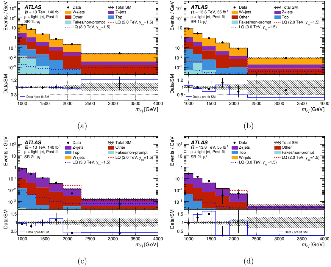
Figure 11. Data (dots) and post-fit SM distribution (histograms) of m_{\ell j} in (a), (b) SR-1L- \mu j and (c), (d) SR-2L- \mu j of the \mu + light-jet channel obtained by a CR+SR background-only fit for Run 2 and Run 3, respectively. The lower panel shows the ratio of observed data to the total post- and pre-fit SM prediction. The last bin includes the overflow. Uncertainties in the background estimates include both the statistical and systematic uncertainties, with correlations between uncertainties taken into account. The dashed lines show the predicted yields for two benchmark signal models corresponding to \tilde{S}_1(m, y_{s\mu}) = (2.0 \text{ TeV}, 1.5) and \tilde{S}_1(m, y_{s\mu}) = (3.0 \text{ TeV}, 1.5) , respectively.
