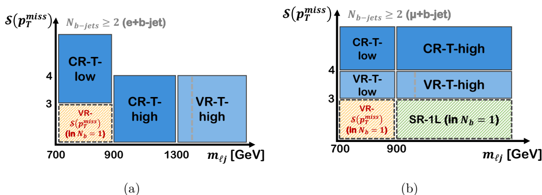
Figure 6. Illustrations of the CRs and VRs definitions for the top background in the (a) e + b\text{-jet} and (b) \mu + b\text{-jet} channel, respectively. The phase spaces of VR- S(p_T^{\text{miss}}) and SR-1L which select event with exactly one b -tagged jet are indicated as hatched boxes. The phase space SR-1L is only indicated in (b) as it overlaps with the phase space of CR/VR-T-high in (a) in the m_{\ell j} - S(p_T^{\text{miss}}) plane. Grey vertical dashed lines indicate that a region is binned in m_{\ell j} .
