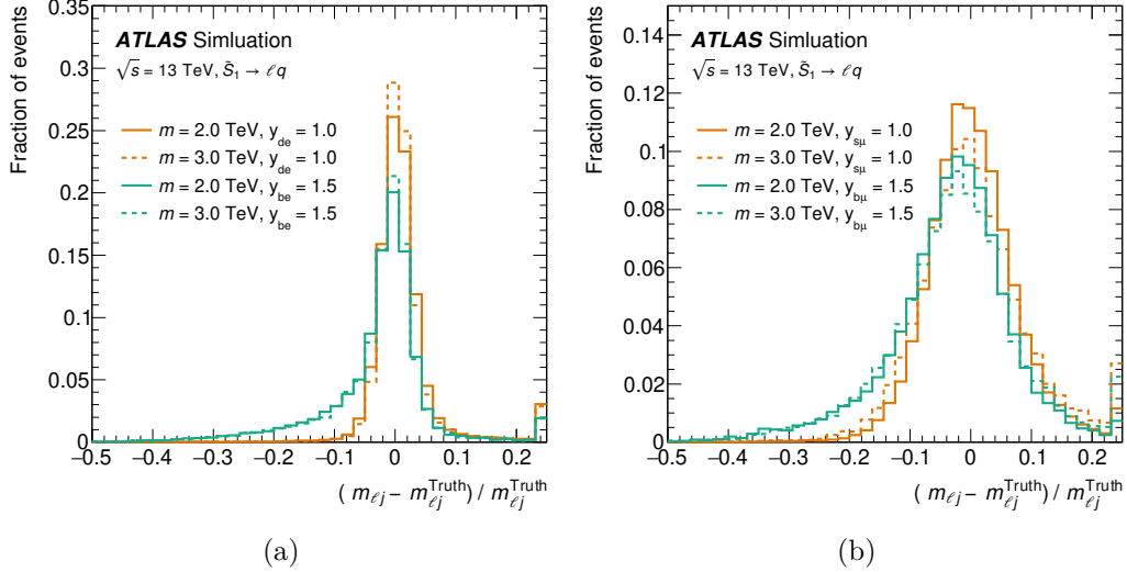
Figure 2. Relative difference between the reconstructed m_{\ell j} and particle-level m_{\ell j}^{\text{Truth}} invariant mass of the lepton-jet system for selected example LQ scenarios in the (a) e + \text{light-jet} and e + b\text{-jet} , and (b) \mu + \text{light-jet} and \mu + b\text{-jet} channels using Run 2 MC simulation. The dashed lines correspond to an LQ scenario with a larger mass but the same coupling as the one shown by the solid lines. The particle-level invariant mass is calculated using the particle-level four-momenta of the reconstructed lepton and jet. The last bin contains the overflow.
