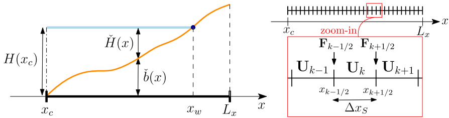
Fig. 3 Left: Fixed shallow-water computational domain (bold line segment) as defined by \bar{\Omega}_S = [x_c, L_x] . The local rest depth \tilde{H}(x) and beach topography \tilde{b}(x) are also illustrated. Right: Discretised shallow-water domain consists of N_v volumes of uniform size \Delta x_S
