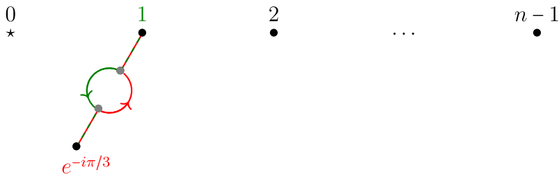
FIGURE 5 The path p_{t_2} associated to the reflection t_2 . Note that only the first two entries of the n -tuple are non-constant paths. The drawing is for d = 3 . For larger d , the endpoints of the paths are closer.
