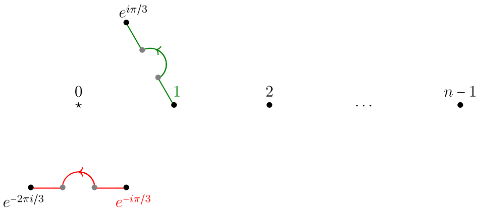
FIGURE 6 The path p_{t'_2} associated to the reflection t'_2 . Note that only the first two entries of the n -tuple are non-constant paths. The drawing is for d = 3 . For larger d , the path starting at e^{-i\pi/3} lies entirely within the fourth quadrant of the plane and the endpoints of both paths are closer.
