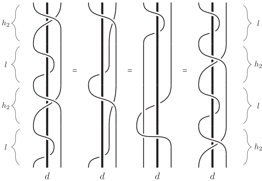
FIGURE 11 The braids lh_2lh_2 on the left and h_2lh_2l on the right are equal.
