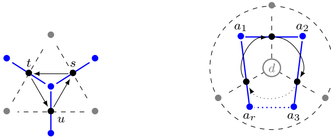
FIGURE 25 Two possible local behaviours appearing in T . The dashed arcs are arcs in T (in the right-hand picture the arcs shown on the boundary are also allowed to be boundary segments). The solid edges are edges in D_T and edges in Q_T are oriented.
