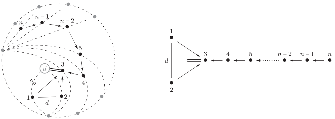
FIGURE 12 Original presentation from [6] (shown on the right) embedded in a disk with n marked points on the boundary and a cone point of degree d in its interior.
