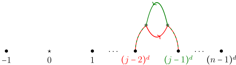
FIGURE 9 Path p_{t_j} to the power d for 3 \leq j \leq n .
