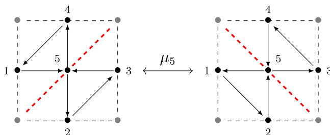
FIGURE 17 A mutation far from the conept.
