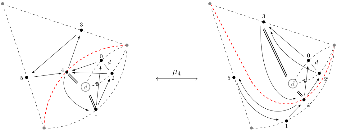
FIGURE 19 A mutation near the cone point.
