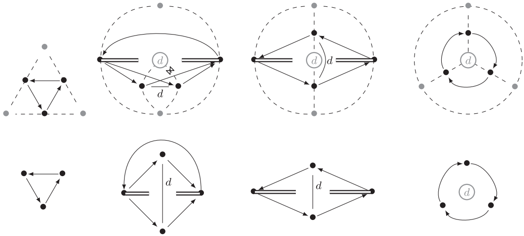
FIGURE 14 Building up the associated quiver for a disk with cone point. We show the corresponding quivers separately. Note that the cone point itself does not appear in the quiver in the second and third cases.
