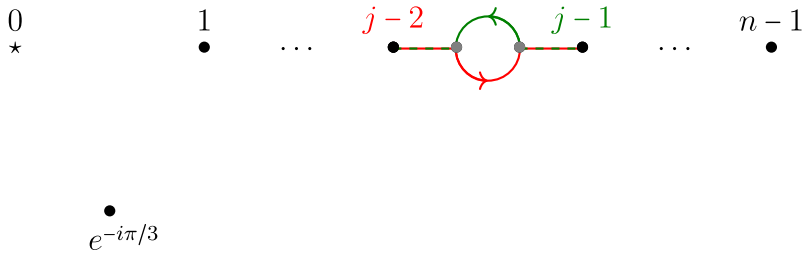
FIGURE 7 The path p_{t_j} associated to the reflection t_j for 3 \leq j \leq n . Note that only the (j-1) st and j th entries of the n -tuple (with initial values j-2 and j-1 , respectively) are non-constant paths. We draw the case d = 3 .
