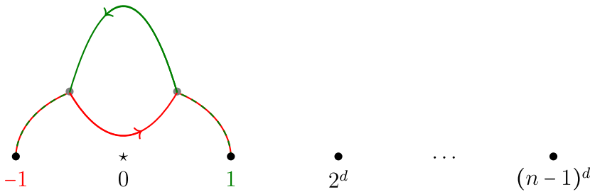
FIGURE 8 Path p_{t'_2} to the power d .
