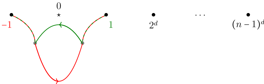
FIGURE 3 Path p_{t_2} to power d .
