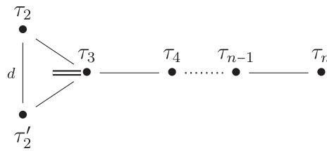
FIGURE 2 The presentation of B(d, d, n) from [6].
