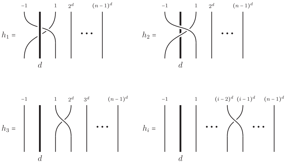
FIGURE 4 The braids h_1, h_2, \dots, h_n . The thicker line (pole) represents the cone point of degree d .
