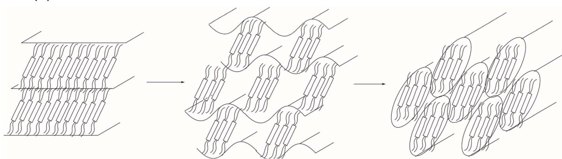
Fig. 22 Figures to show: (a) the organisation in the SmC phase of tetracatenar mesogens and illustrates how the tilted core enables a planar core-chain interface; (b) the effect of increased terminal chain volume in a tetracatenar mesogen leading to undulating layers and finally columnar organisation. Fig. 22a is reproduced from ref. 92; Fig. 22b is adapted with permission from ref. 97. Copyright 2000 American Chemical Society.
