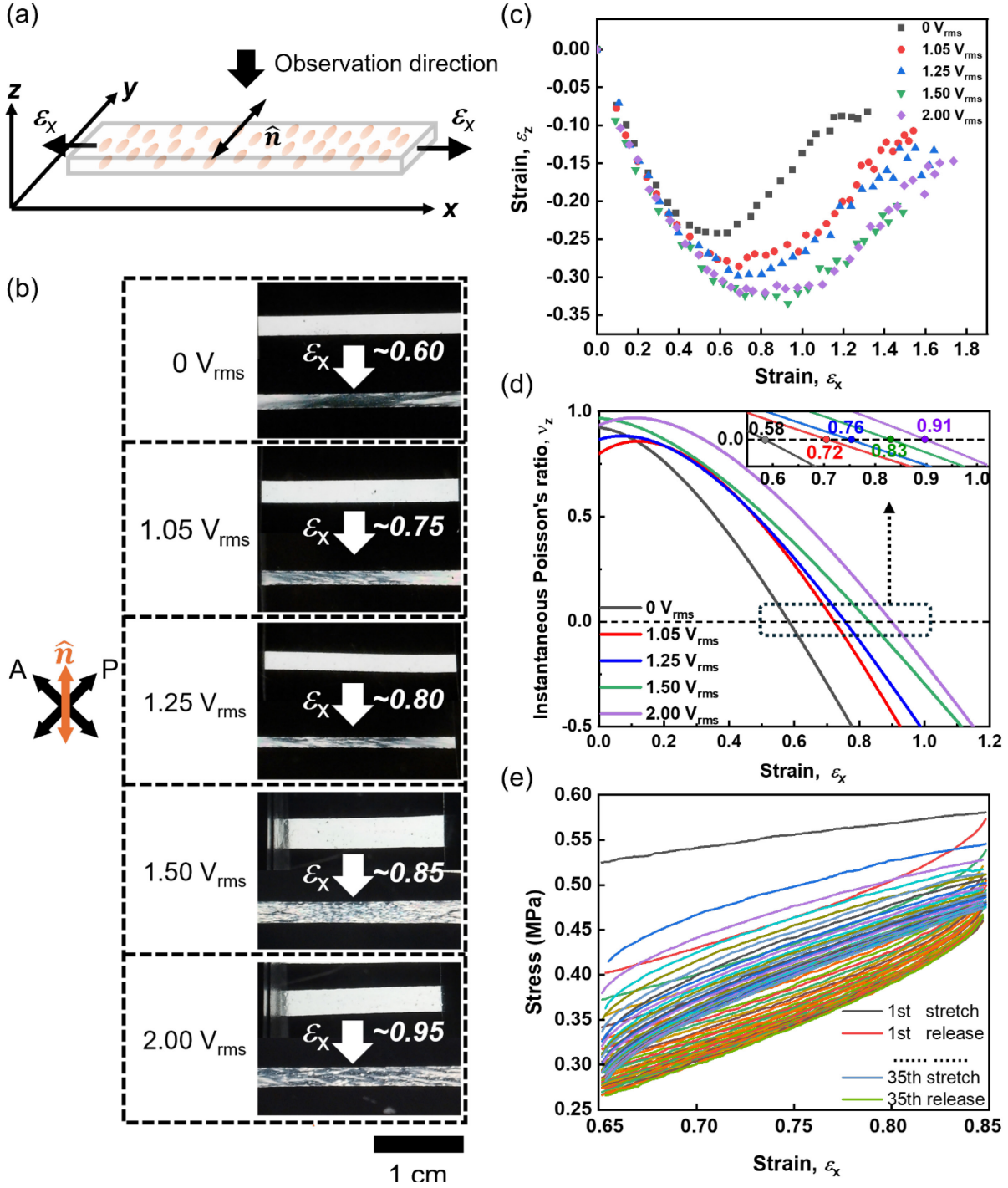
Figure 2. a) The geometry of the undeformed IALCE samples. The projection of the director \hat{n} is parallel to the y -axis and the strain is applied along the x -direction ( \epsilon_x ). The observation direction is along the z -direction. b) The POM images show the initial, unstrained, state and the dark state emerging near the threshold auxetic strain for the IALCE prepared at 0 V_{rms} , 1.05 V_{rms} , 1.25 V_{rms} , 1.50 V_{rms} and 2.00 V_{rms} . The strains of the dark states are indicated, all of which are near though higher than the \epsilon_{th} . The scale bar is 1 cm. c) The strain \epsilon_z as a function of \epsilon_x measured for all the samples. d) The instantaneous Poisson's ratio in the thickness of the film, \nu_z , measured for all the samples. The inset figure shows the crossing of each line at \nu_z = 0 . e) The 35-cycle mechanical measurement of a planar IALCE sample.
