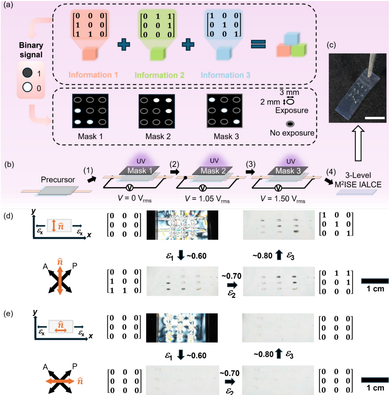
Figure 4. a) Optical information in the format of a binary signal, with 3-level information designed into three masks. Black and white represent '1' and '0'. b) The fabrication process for 2D optical M 2 ISE IALCEs. c) A photograph of the IALCE under white light; scale bar is 1 cm. d) The decryption process with the initial director direction at 45° to the crossed
