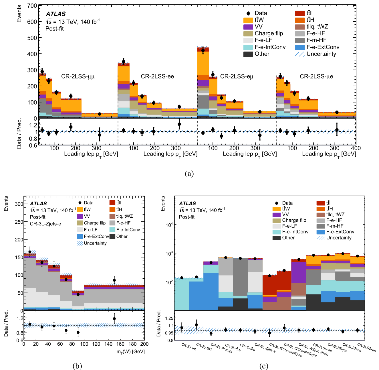
Fig. 3 Event yields as a function of the relevant kinematic variables in a the CR-2LSS CRs, b the CR-3L-Zjets-e CR, and c inclusively in all CRs considered in the analysis after the fit to data. The uncertainty
