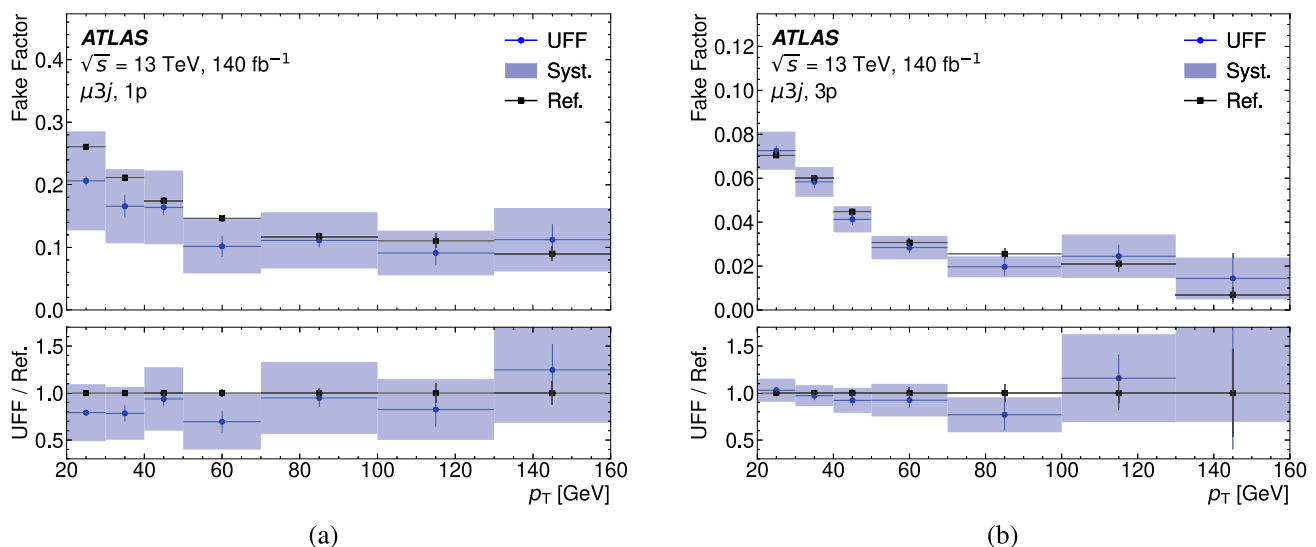
Fig. 13 FFs for the a 1-prong (1p) and b 3-prong (3p) fakes as a function of the fake- \tau_{\text{had-vis}} p_T in the \mu 3j region. Blue-circle points display FFs estimated using the UFF method. The statistical (systematic) uncertainty is displayed as the blue error bars (band). The reference
