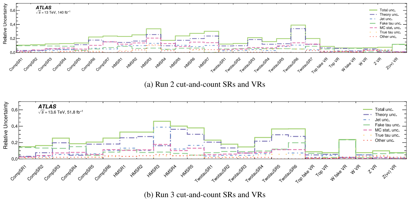
Fig. 10 Comparison of the dominant groups of systematic uncertainties in the total background prediction after the background-only fit for the cut-and-count approach, relative to the total yields. The total uncertainty is calculated using all the available systematic and statistical
