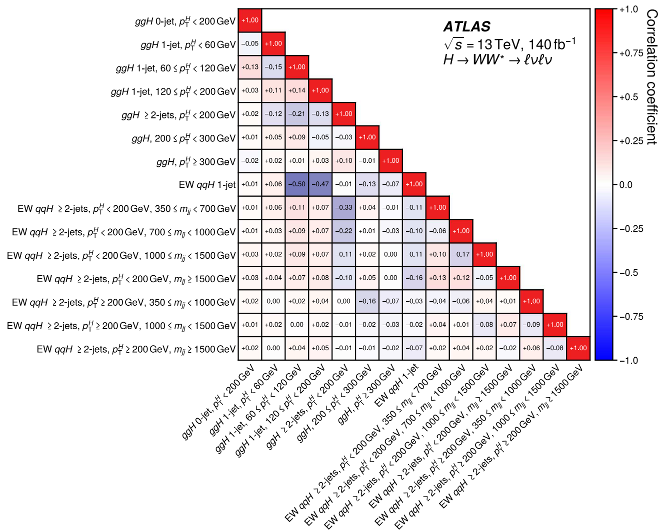
Fig. 19 Observed correlations between the production cross-sections multiplied by the H \rightarrow WW^* branching ratio measured in data for each of the STXS categories, as discussed in Sect. 10.1
