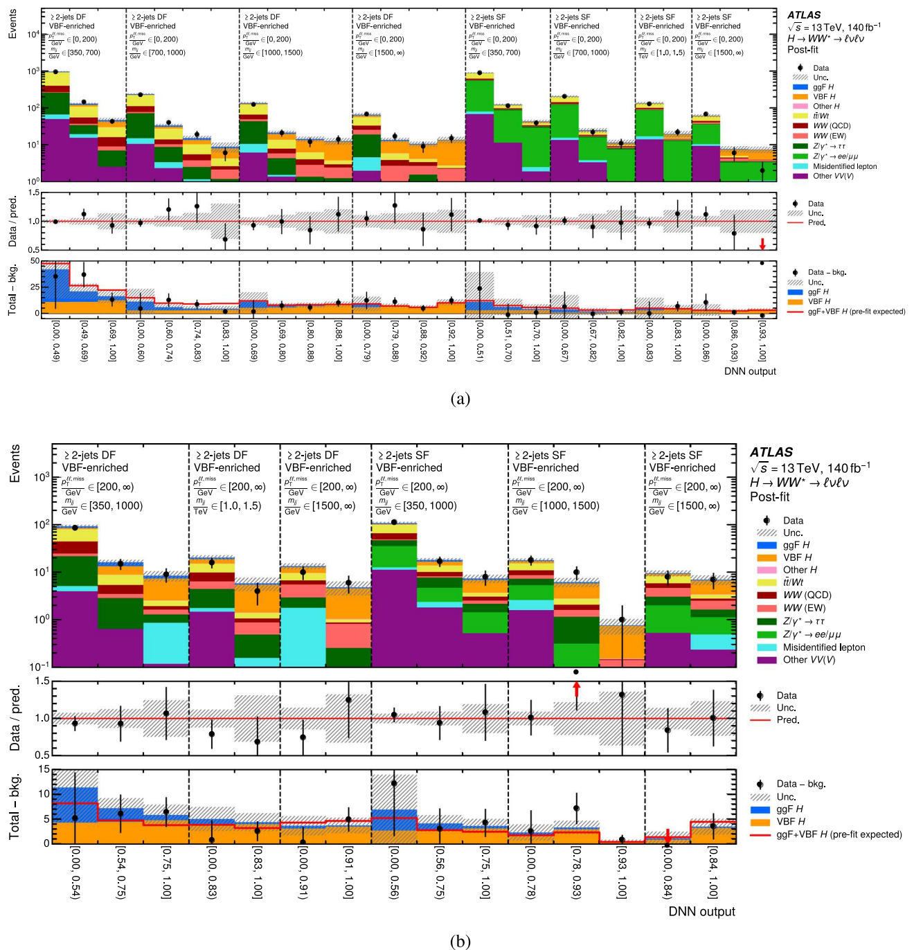
Fig. 9 Post-fit DNN distributions in the VBF \geq 2-jets a low and b high p_{T}^{\ell\ell, \text{miss}} SRs entering the STXS measurement for both the DF and SF channels; the post-fit results are obtained from the 15-POI fit. The vertical dashed lines delineate different SRs. The middle panels show the ratios of the data to the sum of the fitted signal and background, and the bottom panels show the differences between
