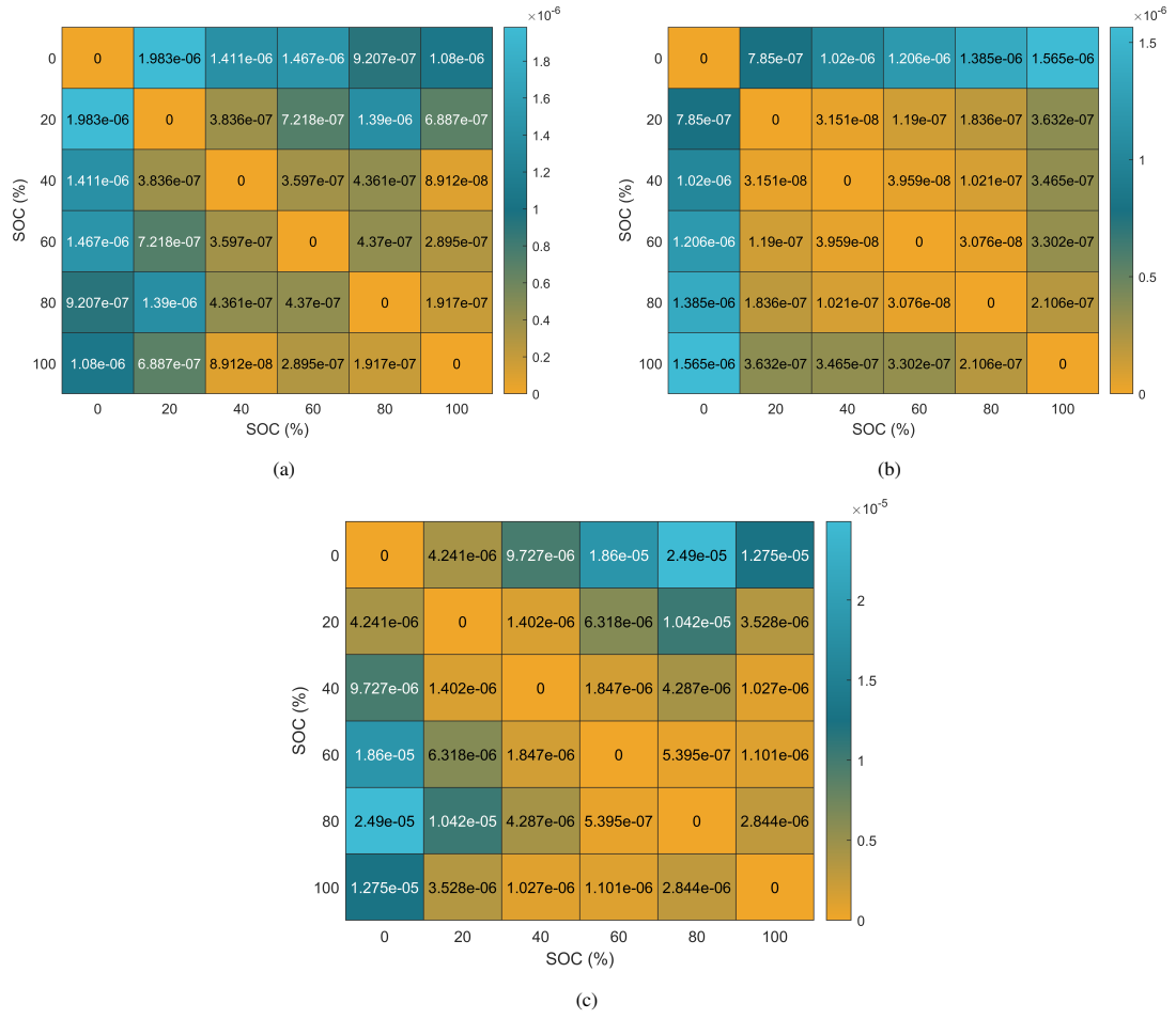
Figure 1: The mean square error (MSE) for all SOC% for a) Cell 1, b) Cell 2, and c) Cell 3.
