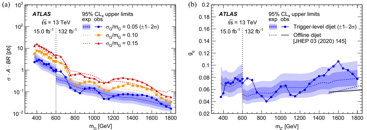
FIG. 9. Observed 95% CL s upper limits on (a) the production cross section times acceptance times branching ratio to jets, \sigma \cdot A \cdot BR , of Gaussian-shaped signals of 5% (filled circles), 10% (squares) and 15% (triangles) width relative to their peak mass, m_G , and (b) the value of the coupling to quarks, g_q , of the Z' model as a function of the resonance mass m_{Z'} (filled circles). Also shown are the corresponding expected upper limits predicted for the case the m_{jj} distribution is observed to be identical to the background prediction in each bin (dashed lines). For the narrowest Gaussian-shaped (5%) and Z' signals, the shaded bands indicate the 1\sigma (darker band) and 2\sigma (lighter band) envelopes of outcomes expected for Poisson fluctuations around the background expectation. The uncertainty bands for wider Gaussian-shaped signals are of similar relative size. Overlaid on panel (b) are the observed (darker solid line) and expected (darker dashed line) upper limits from the ATLAS Run-2 search using the main stream and offline jets [13], which benefits from tracking information and data in the tile gap region of the calorimeter. Limits are derived independently from the J50 and J100 samples for m_{jj} below and above 600 GeV, respectively, denoted by the vertical dashed line, as discussed in the text.
