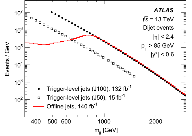
FIG. 2. Distributions of dijet invariant mass m_{jj} for events collected via the TLA stream and reconstructed in the HLT, combining events selected at L1 by the p_T > 100 GeV trigger (filled circles) and the prescaled single-jet and dijet p_T > 50 GeV triggers (open squares), showing the increase in events recorded at lower values of dijet mass for this analysis compared with events collected via the main stream and reconstructed offline (histogram). For this illustrative comparison, each sample must satisfy the analysis selection described in Sec. V, except for rejection of the tile gap region, and includes events with at least two trigger or offline jets, each with p_T > 85 GeV and |\eta| < 2.4 , with half a rapidity difference smaller than 0.6. The final sample used for the search is discussed and shown separately in Sec. V.
