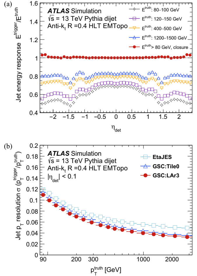
FIG. 5. (a) Trigger jet energy response, E^{\text{trigger}}/E^{\text{truth}} , in bins of detector pseudorapidity \eta^{\text{det}} of the truth jet p_T , p_T^{\text{truth}} , before applying the EtaJES calibration step (open markers in ranges of truth jet energy from 80 to 1500 GeV) and closure after applying the correction (filled circles). (b) Resolution \sigma(p_T^{\text{trigger}}/p_T^{\text{truth}}) of trigger jet transverse momentum p_T as a function of truth jet p_T after the EtaJES calibration step (open squares) and after each of the calorimeter-based GSC steps, Tile0 (open triangles) and LAr3 (filled circles) in the central detector \eta bin |\eta^{\text{det}}| < 0.1 .
