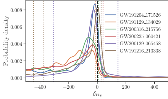
FIG. 9. The posterior probability distribution on the spin-induced quadrupole moment parameter, \delta\kappa_s from the events listed in the SIM column of Table II, passing the selection criteria described in Section V B. The black dashed vertical line indicates the BBH value ( \delta\kappa_s = 0 ). The colored vertical lines show the 90% symmetric bounds on \delta\kappa_s calculated from the individual events assuming a uniform prior ranging between [-500, 500] on \delta\kappa_s .
