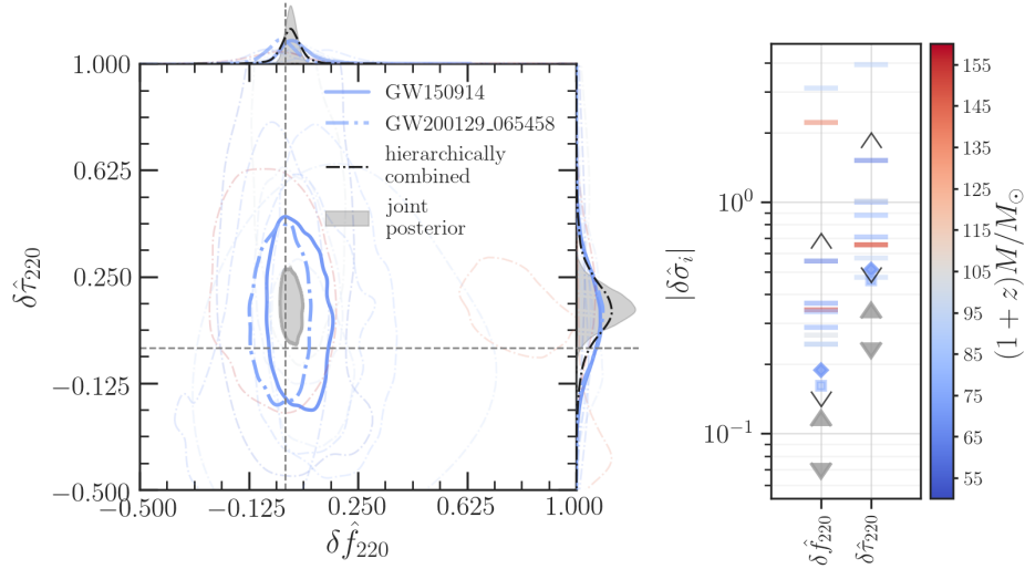
FIG. 14. Left panel: The 90% credible levels of the posterior probability distribution of the fractional deviations in the frequency and damping time of the (2, 2, 0) QNM, (\delta f_{220}, \delta \tau_{220}) and their corresponding one-dimensional marginalized posterior distributions, for events from O1, O2 and O3 passing a SNR threshold of 8 in both the pre- and post-merger signal. Posteriors for GW150914 and GW200129_065458 are separately shown. The joint constraints on (\delta f_{220}, \delta \tau_{220}) obtained multiplying the posteriors (given a flat prior) from individual events are given by the filled grey contours, while the hierarchical method of combination yields the black dot dashed curves in the one-dimensional marginalized posteriors. Right panel: 90% credible interval on the one-dimensional marginalised posteriors on \delta \sigma_i = (\delta f_{220}, \delta \tau_{220}) , colored by the median redshifted total mass (1+z)M , inferred assuming GR. Filled gray (unfilled black) downward triangles mark the constraints obtained when all the events are combined by multiplying posteriors (hierarchically). For comparison, we mark the previously published bounds from [11] using filled/unfilled upward triangles. The bounds from GW200129_065458 (square) and GW150914 (diamond) are indicated by the separate markers. See Sec. VIII A 2 for details.
