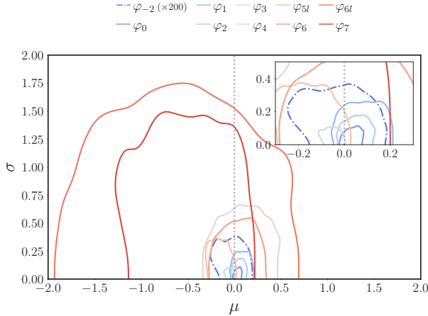
FIG. 8. Joint distribution for the hyperparameters \mu and \sigma of the GR deviation coefficients for the parametrized tests on generic gravitational-wave modifications of Sec. V A. Contours mark 90% credible regions and they all include \mu = \sigma = 0 , which corresponds to the GR prediction. These results were obtained with a pipeline based on SEOBNRv4_ROM. The \phi_{-2} -contour has been rescaled by a factor of 200 to improve visibility, as deviations for this term are the most tightly constrained. Warm (cold) colors refer to deviations occurring at higher (lower) PN orders.
