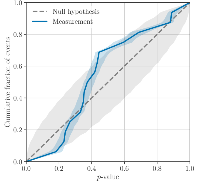
FIG. 15. Results of the echoes analysis (Sec. VIII B). Plot of fraction of events for which the echoes signal-to-noise p -value is less than or equal to the abscissa. The light-blue band represents the 90% credible interval of the observed p -values, while the diagonal dashed line is expectation from the null hypothesis. The light-gray band around the diagonal line represents the 90% uncertainty band of the null hypothesis.
