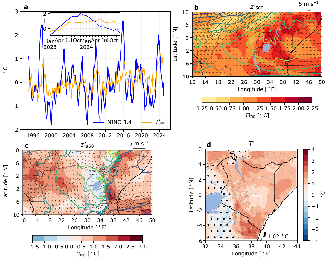
Figure 3. (a) 1995–2024 time series of the monthly El-Niño Southern Oscillation 3.4 index (NINO 3.4, blue line) and the pan-Tropical (30°S–30°N, 180°W–180°E) monthly mean temperature anomaly at 500hPa ( T'_{500} , orange line) with respect to the 1995–2024 average. The inset shows the 2023–2024 period. 15–20 February 2024 daily anomaly averages of (b) geopotential height (contours, in m), temperature (shading, in °C) and total wind speed (vectors, in \text{ms}^{-1} ) at 500hPa. (c) Same as (b) but at 850hPa. (d) 15–20 February 2024 daily anomaly averages of near-surface temperature ( T' ); the domain-average anomaly is indicated in the bottom right corner; anomalies significant at the 5% level are not stippled; orography is denoted with grey contours (see Figure 1a for elevation values).
