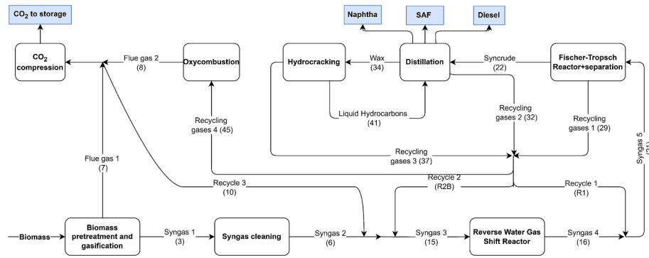
Fig. 5. Flow of carbon throughout the main process units of the refinery plant. (In parentheses, the stream names as labelled in Fig. 1).
