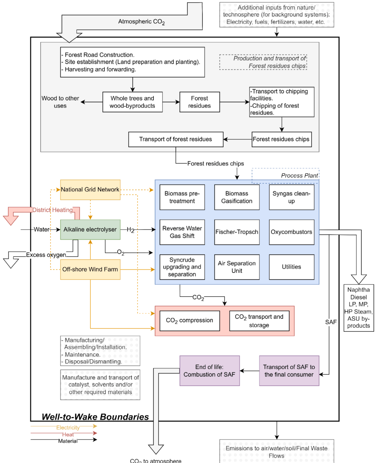
Fig. 3. Well-to-Wake boundaries of the life cycle assessment of the PBtL-CCS scenarios.
