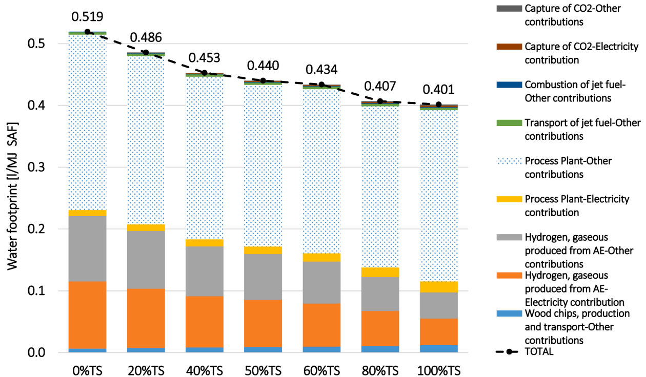
Fig. 14. Water footprint breakdown for the different scenarios.
