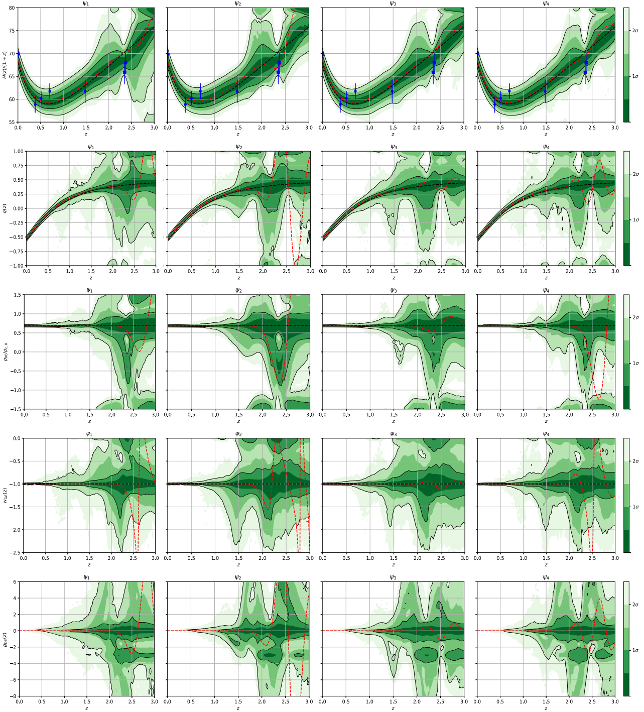
Figure 5. Functional posterior probability of H(z)/(1+z) , q(z) , \rho_{DE}(z)/\rho_{c,0} , w_{DE}(z) , and q_{DE}(z) for the data sets SB + SN . The probability, normalized in each slice of constant z , is shown with a color scale representing confidence interval values. The 68 per cent ( 1\sigma ) and 95 per cent ( 2\sigma ) confidence intervals are plotted as black lines. The dashed black line corresponds to the standard \Lambda CDM values, and the dashed red line represents the best-fitting values of the wavelets. These plots were made using the PYTHON library fgivenx (W. Handley 2018).
