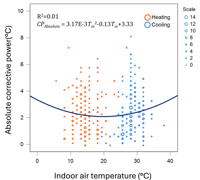
Fig 10. Relation between absolute corrective power and indoor air temperature.
