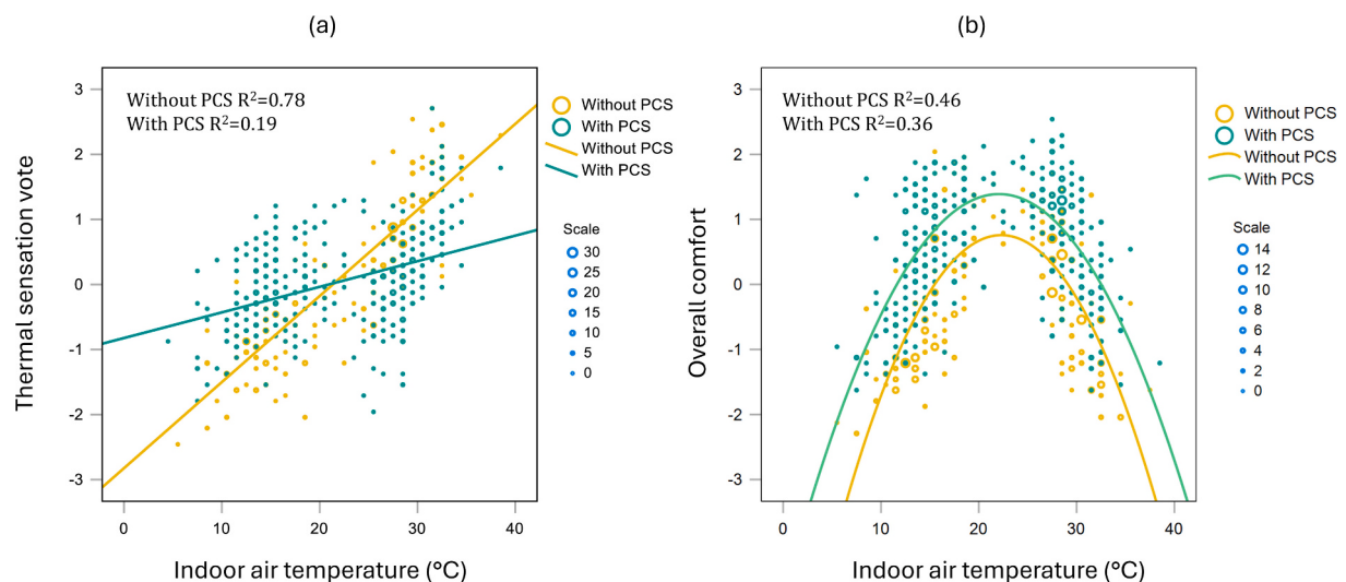
Fig 7. Relationship between thermal responses and indoor air temperature for with and without PCS conditions: (a) Thermal sensation and (b) Overall comfort.
