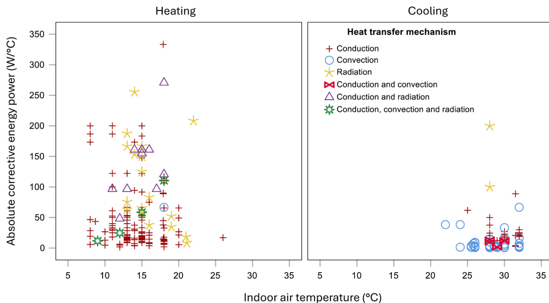
Fig 11. Absolute corrective energy power values for each indoor air temperature.
