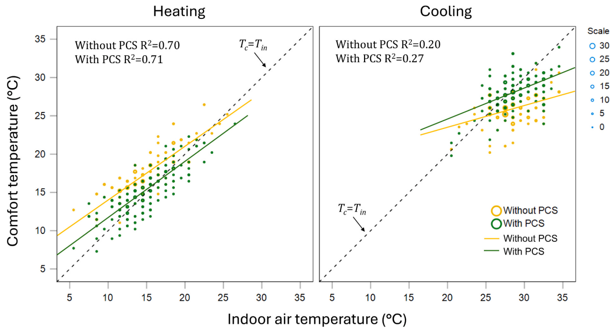
Fig 9. Relationship between the comfort temperature and indoor air temperature.
