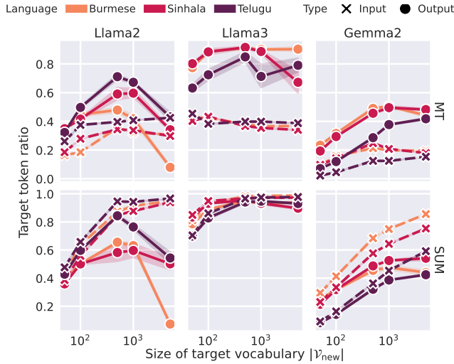
Figure 4 Average target token ratio in input (x) and output (•) with respect to |\mathcal{V}_{new}| across models, languages, and tasks.
