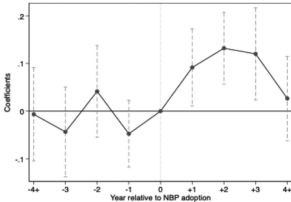
FIGURE 1 | Dynamics of the treatment effect.
