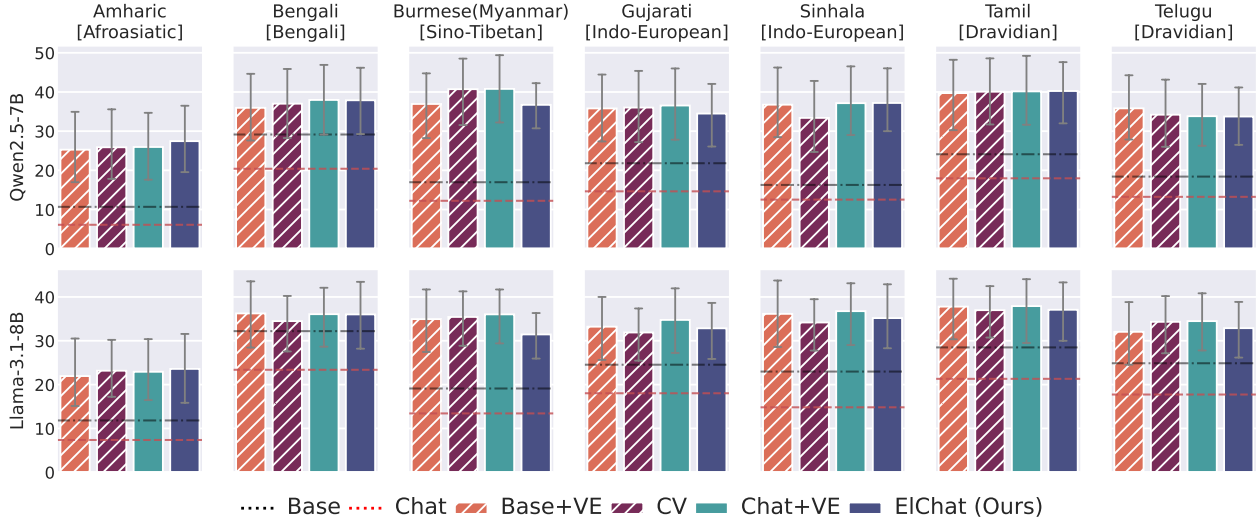
Figure 9: Aggregated mean performance across target language tasks for each model by language (error bars indicate 95% confidence interval).
