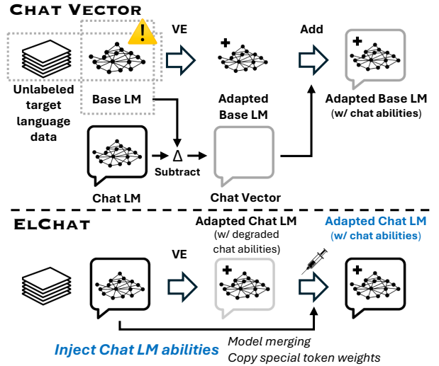
Figure 1: Chat LLM language adaptation with Chat Vector (Huang et al., 2024) and ElChat (ours). Note that a base LM in this paper refers to an LM pre-trained on unlabeled data without any further post-training. A chat LM, on the other hand, is a base model that has been further supervised fine-tuned on labeled conversational data, enabling it to follow instructions.
