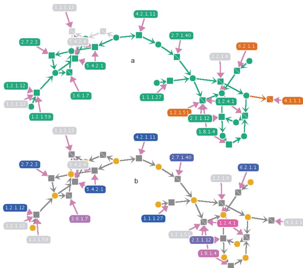
Figure 1. (a) A section of the glycolysis pathway from an automated metabolic reconstruction of the human malaria parasite P. falciparum , visualized using SHARKview. Metabolites are represented as circles, reactions as squares and enzymes as round-edged rectangles. Directed arcs between nodes show the effect of a reaction as the consumption and production of different metabolites. Nodes in green show reactions catalysed by enzymes for which good evidence has been found in the P. falciparum genome. Nodes in red show reactions catalysed by enzymes for which only tentative evidence has been found. Grey nodes show that no evidence for a catalysing enzyme was found. (b) The same pathway section for P. falciparum , with the enzyme nodes coloured according to their level of co-expression with lactate dehydrogenase (EC 1.1.1.27). Blue nodes show a high positive co-expression, whereas a colour towards pink shows a high negative co-expression.
