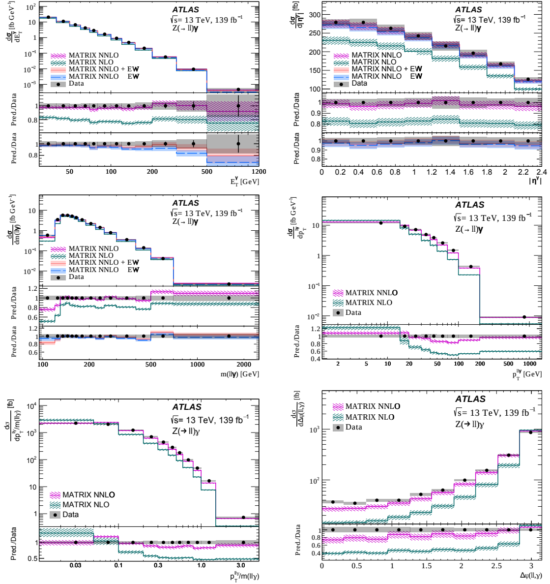
Figure 7. Measured fiducial cross-sections (black data points) for the observables (from left to right and top to bottom) E_T^\gamma , |\eta^\gamma| , m(\ell\ell\gamma) , p_T^{\ell\gamma} , p_T^{\ell\gamma}/m(\ell\ell\gamma) and \Delta\phi(\ell\ell, \gamma) for the pp \rightarrow Z(\ell^+\ell^-)\gamma process. The measured cross-sections are compared with SM expectations obtained from the MATRIX parton-level generator, corrected to particle level. The error bars on the data points show the statistical uncertainty in the measured values. The grey shaded regions show the total uncertainty in the unfolded data, excluding the uncertainty in the integrated luminosity. The purple and green hatched regions show the total uncertainty in the MATRIX predictions. For the quantities E_T^\gamma , |\eta^\gamma| and m(\ell\ell\gamma) , the blue (orange) histograms show the MATRIX NNLO cross-sections with EW NLO corrections applied multiplicatively (additively), while the blue (orange) shaded regions show the corresponding total uncertainties. The lower panel(s) in each plot show the ratio of the SM expectation to the measured cross-section.
