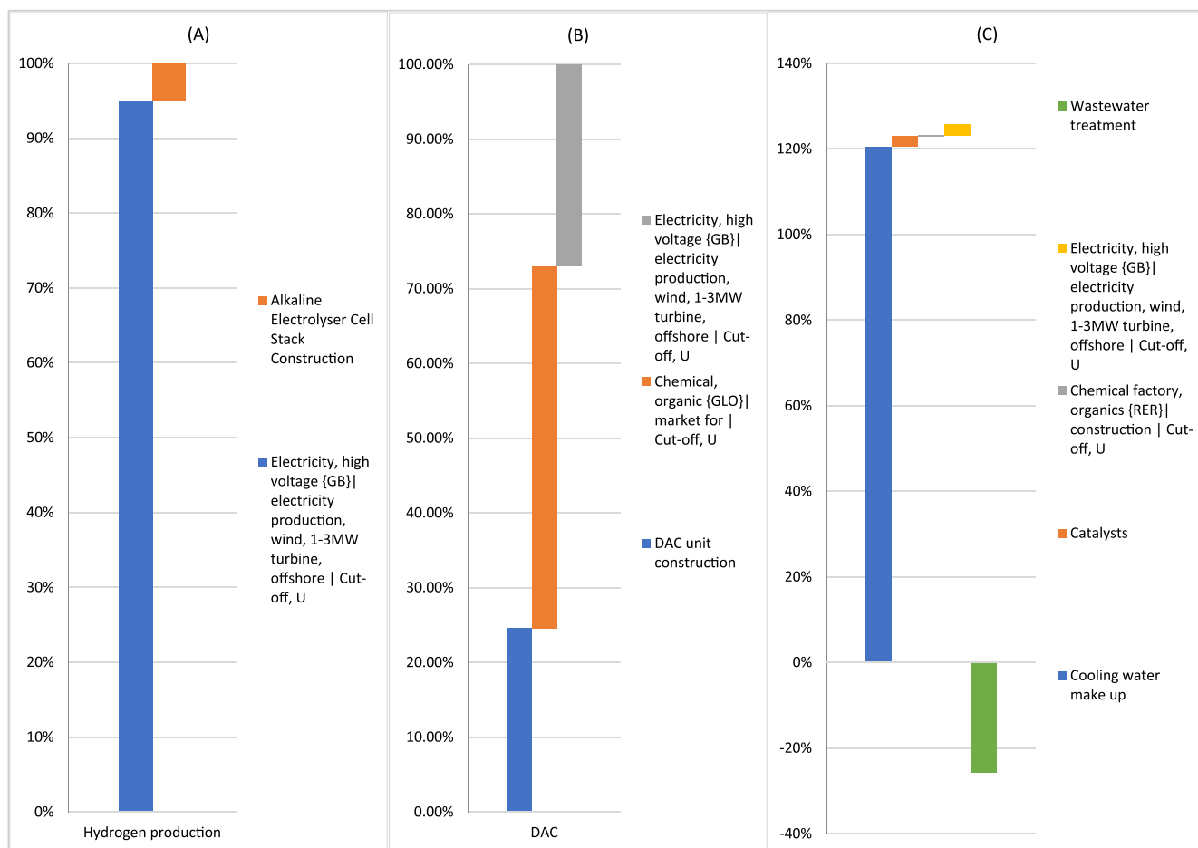
Fig. 16. The breakdown of the Water Footprint: A) hydrogen production stage. B) Direct Air Capture. C) Refinery plant.
