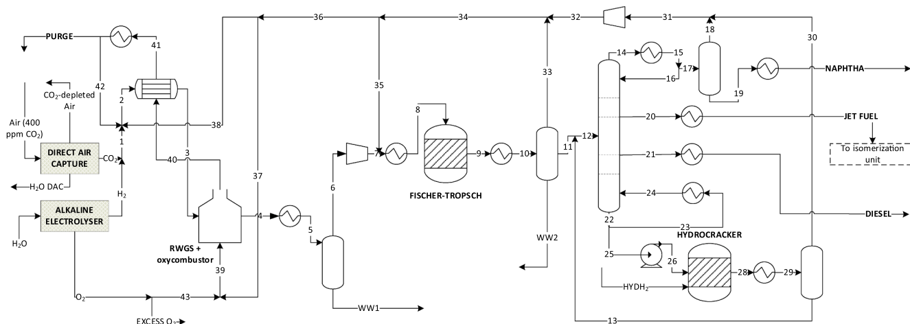
Fig. 1. Process flow diagram of the investigated PtL process for SAF production.
