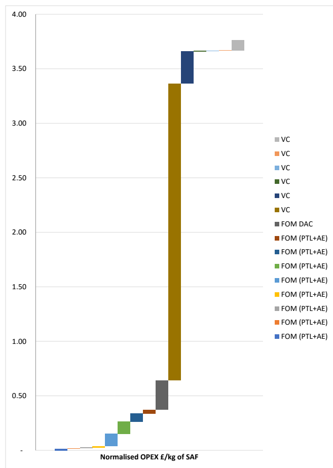
Fig. 6. The normalised OPEX of the investigated SAF route.
