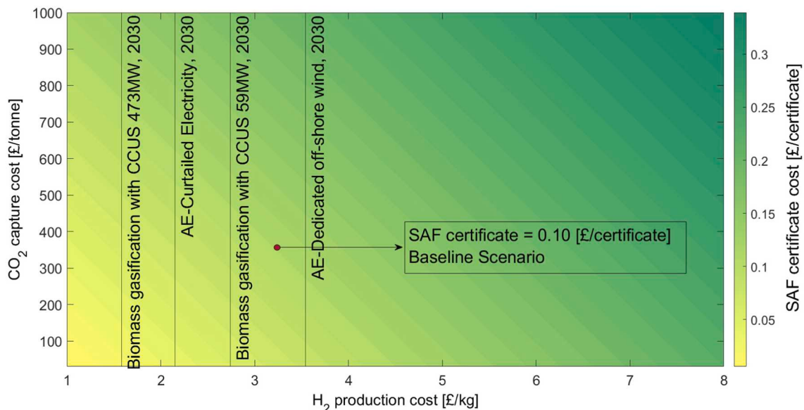
Fig. 18. The SAF certificate cost for the MJSP to break-even with fossil jet fuel cost (0.56£/kg) for different CO 2 capture and H 2 production costs.
