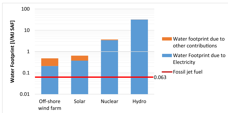
Fig. 17. Water footprint of the PtL-SAF when connected to different electricity sources.
