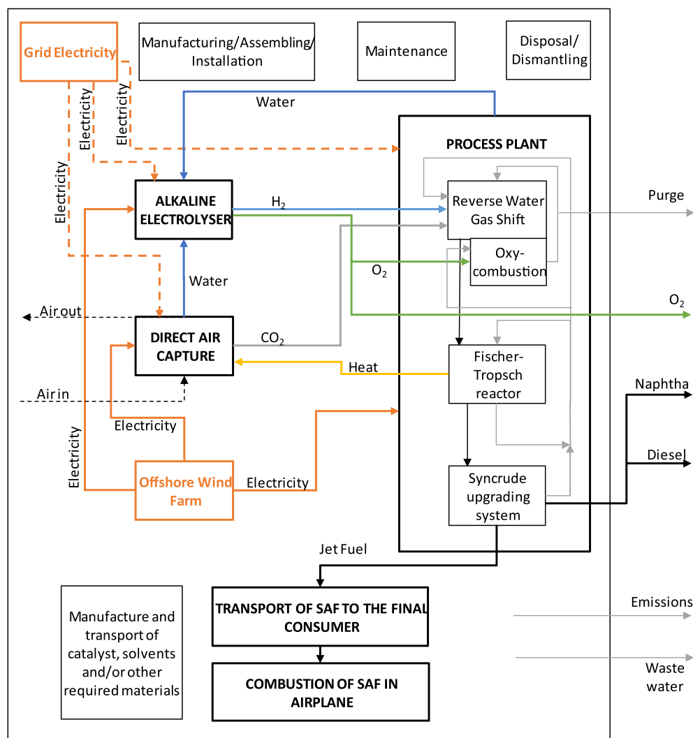
Fig. 3. The system boundaries for the LCA of the investigated SAF route.
