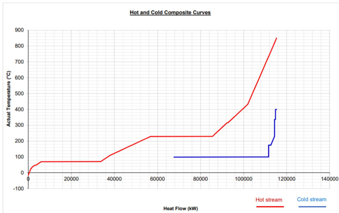
Fig. 5. The composite curves of the PtL system.
