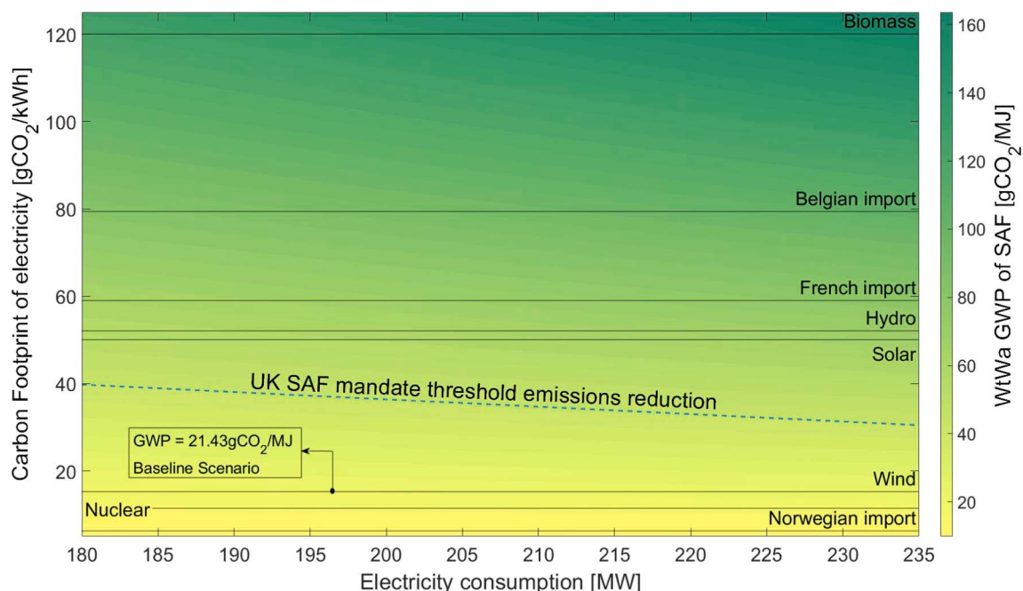
Fig. 13. The GWP of the WtWa life cycle of SAF for different electricity sources at different PtL electricity consumption.
