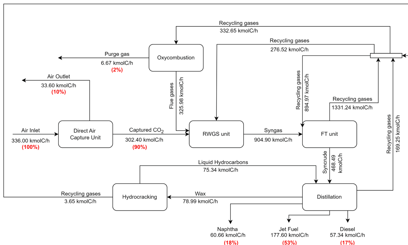
Fig. 4. The carbon mole flow of the investigated SAF route.
