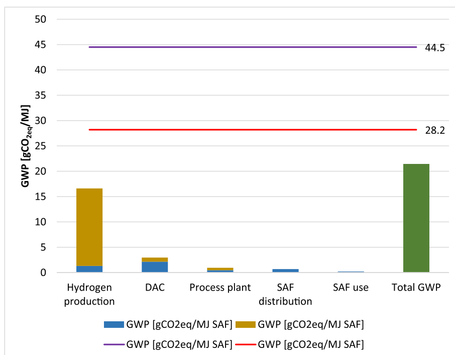
Fig. 11. The contribution of electricity for each process stage, the overall GWP and comparison with existing sustainability standards.
