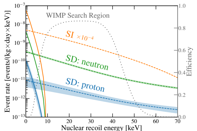
FIG. 1. Comparison of the WIMP-nucleus recoil spectra in the SD neutron-only (green), SD proton-only (blue), and SI (orange, scaled by 10^{-4} ) cases in LXe for a 10 \text{ GeV}/c^2 (solid curve) and 100 \text{ GeV}/c^2 (dashed curve) WIMP and a WIMP-nucleon cross section of 10^{-45} \text{ cm}^2 . The bands on the SD spectra come from uncertainties in the contribution to SD scattering from interactions involving the exchange of a pion between two nucleons (two-body currents). The WIMP search region in XENON1T is depicted by the total efficiency curve (gray dotted).
