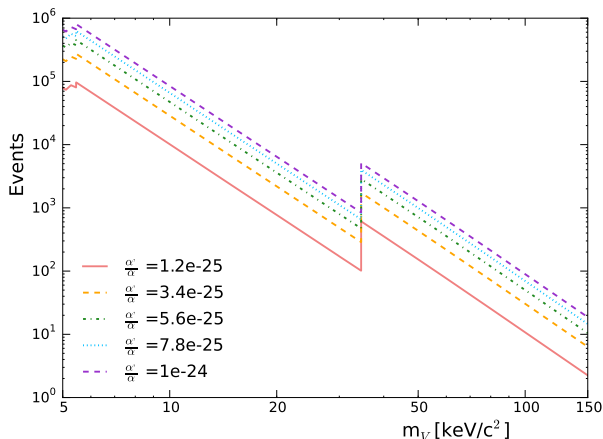
FIG. 1. Predicted total number of events, assuming an infinite energy resolution, for vector super-WIMPs in XENON100 as a function of mass for a range of coupling constants. The assumed exposure is 34 \text{ kg} \times 225 live days of data.
