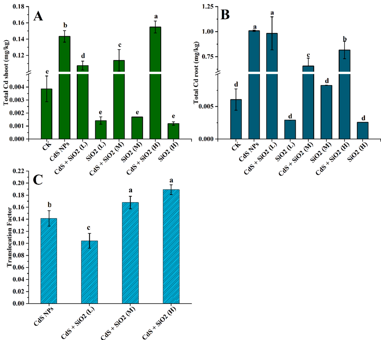
Fig. 1. Total Cd in spinach plant after CdS NPs, SiO 2 and co-exposure (A) shoots (B) roots. Translocation factor (TF) is shown in (C). The results of four replicate samples were presented as mean \pm SD. Different bars represent the significant difference ( p < 0.05 ).
