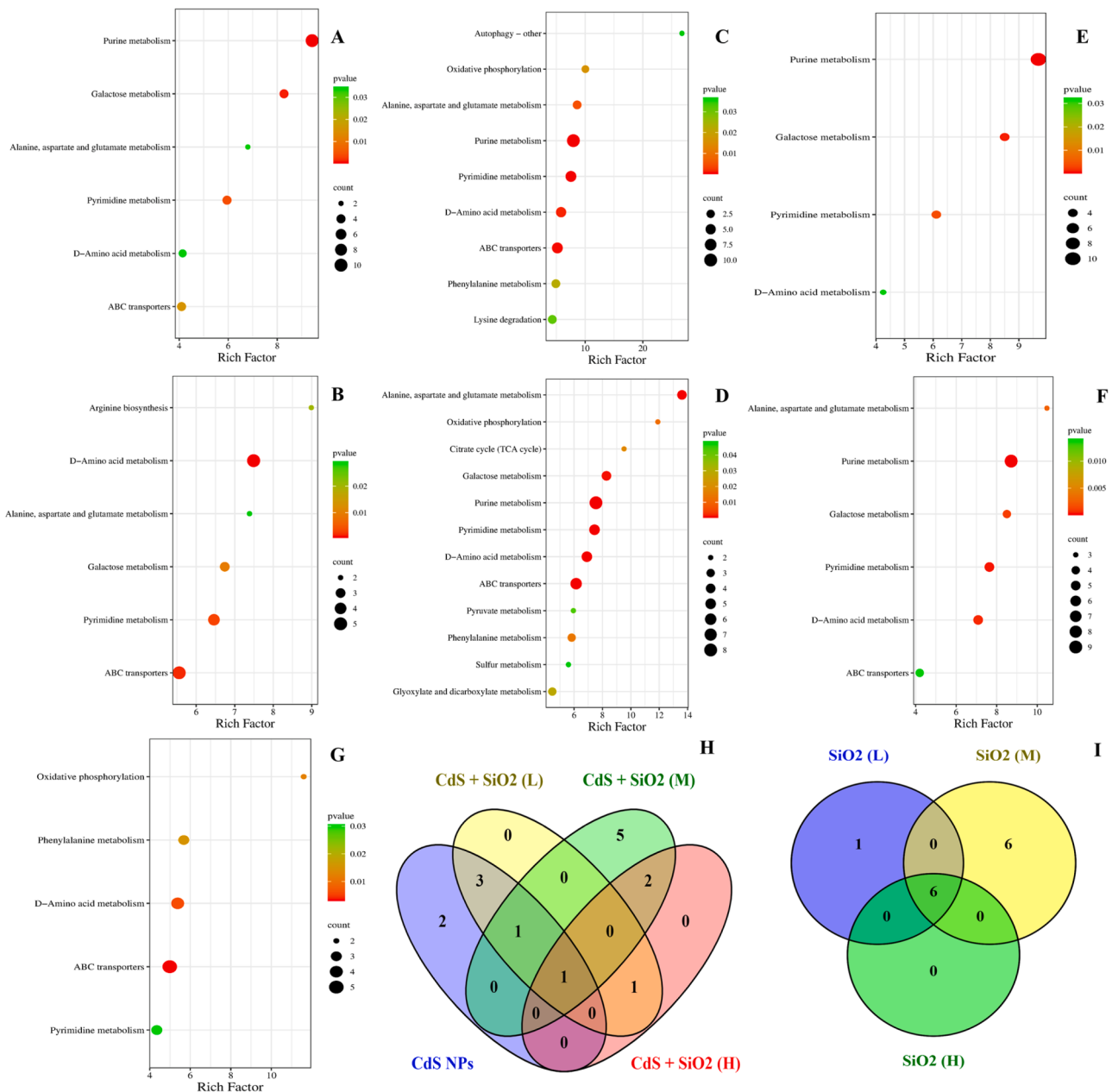
Fig. 5. Metabolic pathways induced by the discriminating metabolites in (A) CdS + SiO 2 (L), (B) SiO 2 (L), (C) CdS + SiO 2 (M), (D) SiO 2 (M) (E) CdS + SiO 2 (H), (F) SiO 2 high dose and (G) CdS VS CG. (H) overlapped metabolites in co-exposure groups and (I) only exposure to SiO 2 NPs.
