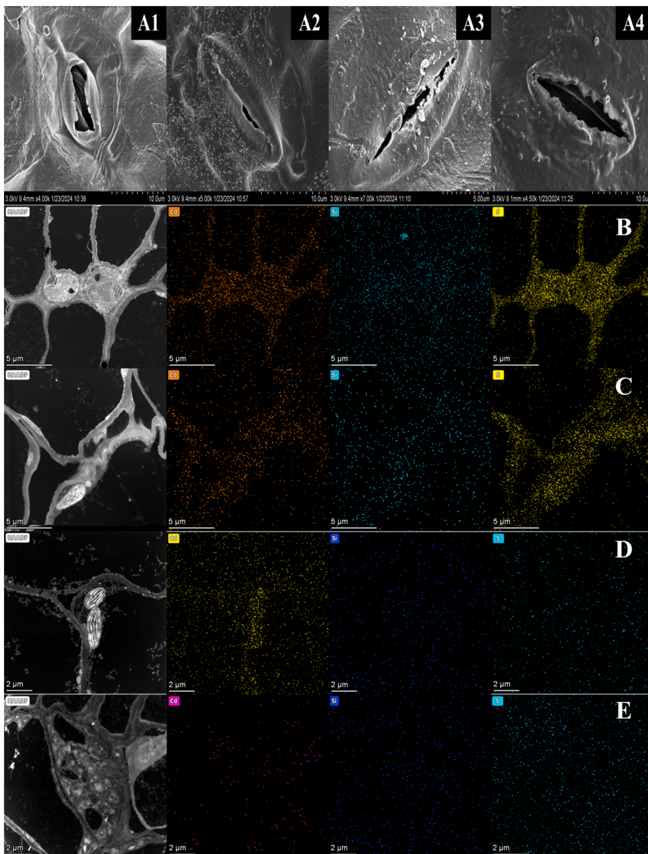
Fig. 2. SEM images of stomata (A1) CG, (A2) CdS, (A3) co-exposure, (A4) SiO 2 , TEM images (B) shoots with co-exposure, (C) roots with co-exposure, (D) shoots with CdS, and (E) roots with CdS exposure.
