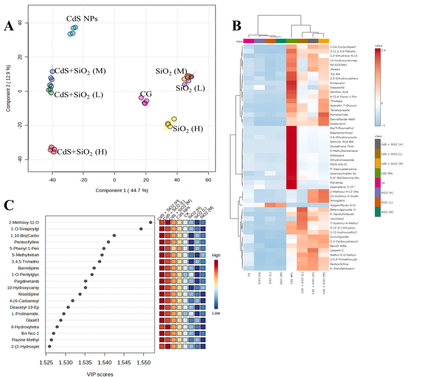
Fig. 4. (A) The PLS-DA score plot displays the separation and clustering of treatment groups based on metabolomic profiles, (B) heat map of relative abundance of the top 50 metabolites across all treatment groups. Rows represent metabolites, columns represent samples, and color gradients indicate concentration levels for comparison between treatment. (C) shows the top 20 metabolites (VIP > 1.5), highlighting the most significant metabolites for distinguishing between treatment groups, with VIP scores from the PLS-DA model indicating their importance.
