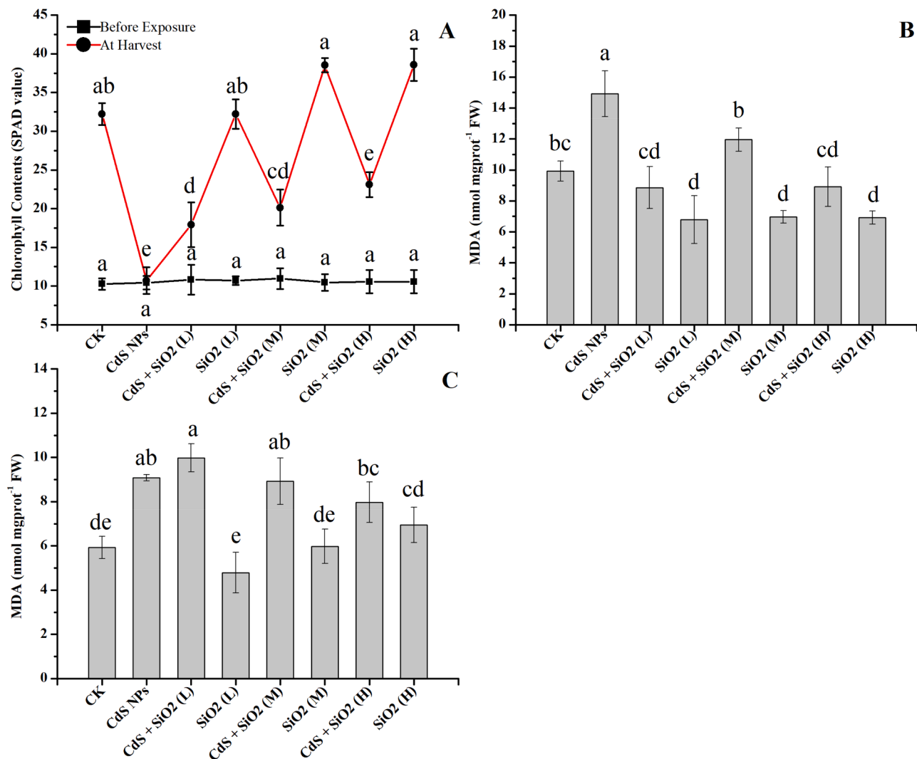
Fig. 3. (A) Relative chlorophyll content in different treatments: CdS, co-exposure and SiO 2 low, medium, and high doses for spinach, before exposure and after exposure. MDA level in (B) leaves and in (C) roots. Significant differences between the treatment means are shown by bars with different letters ( p < 0.05 ). Data are reported as the mean \pm SD ( n = 4 ).
