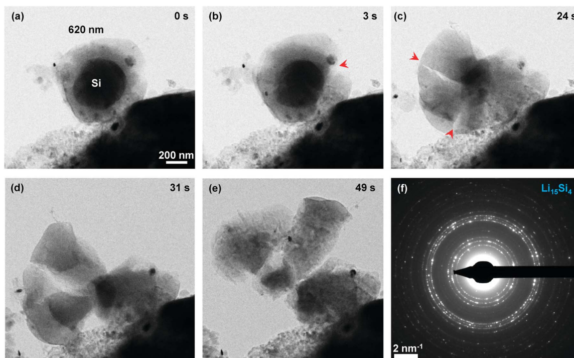
Fig. 2 (a–e) Lithiation of a 620 nm crystalline silicon particle with decrepitation. Red arrows indicate cracks. (f) Electron diffraction indicating the formation of polycrystalline Li_{15}Si_4 upon lithiation. Images reproduced from ref. 10.
