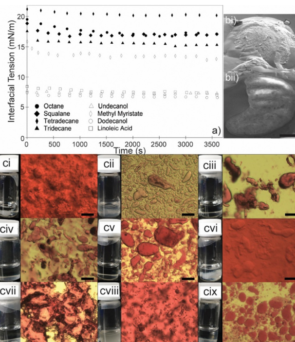
Fig. 2 (a) Interfacial tensions (IFTs) as measured by pendent drop tensiometry of 25 wt% poly(vinyl) alcohol (PVA) aqueous solution suspended in oil containing 2.5 wt% \text{SiO}_2 -NPs. (bi) Cryo-SEM micrographs of Pickering emulsions produced from dispersing PVA based DL in squalane, (bii) emulsion after focused-ion beam, exposing internalised PVA, scale bar is 2.5 \mu\text{m} . (c) Pickering emulsions prepared by dispersing rhodamine B containing DL into oil phases: (ci) undecanol, (cii) methyl myristate, (ciii) squalane, (civ) tetradecane, (cv) tridecane, (cvi) dodecanol, (cvii) pentane, (cviii) linoleic acid, (cix) octane (DL/oil, 20/80 wt%). Scale bars are 50 \mu\text{m} and photographs are PBCA formation 14 h after dissolving BCA in each oil.
