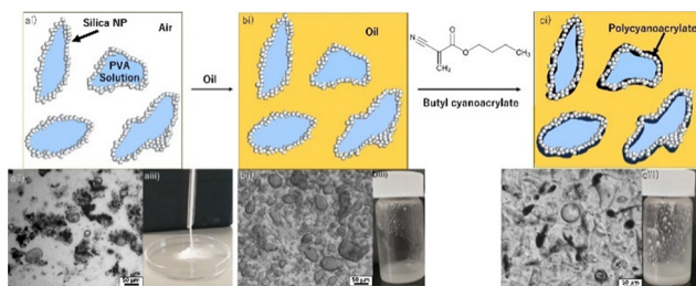
Fig. 1 (ai) Production of dry liquid (DL) via blending 25 wt% poly(vinyl alcohol) aqueous solution with hydrophobised \text{SiO}_2 nano particles. (bi) Dispersion of DL in oil phase to form Pickering-type water-in-oil emulsion. (ci) Addition of butyl 2-cyanoacrylate in oil solution to form a poly(butyl 2-cyanoacrylate) (PBCA) interfacial film via anionic polymerization, which results in formation of microcapsules. (aii)–(cii) Optical micrograph corresponding to respective steps. (aiii)–(ciii) Digital photographs corresponding to respective steps.
