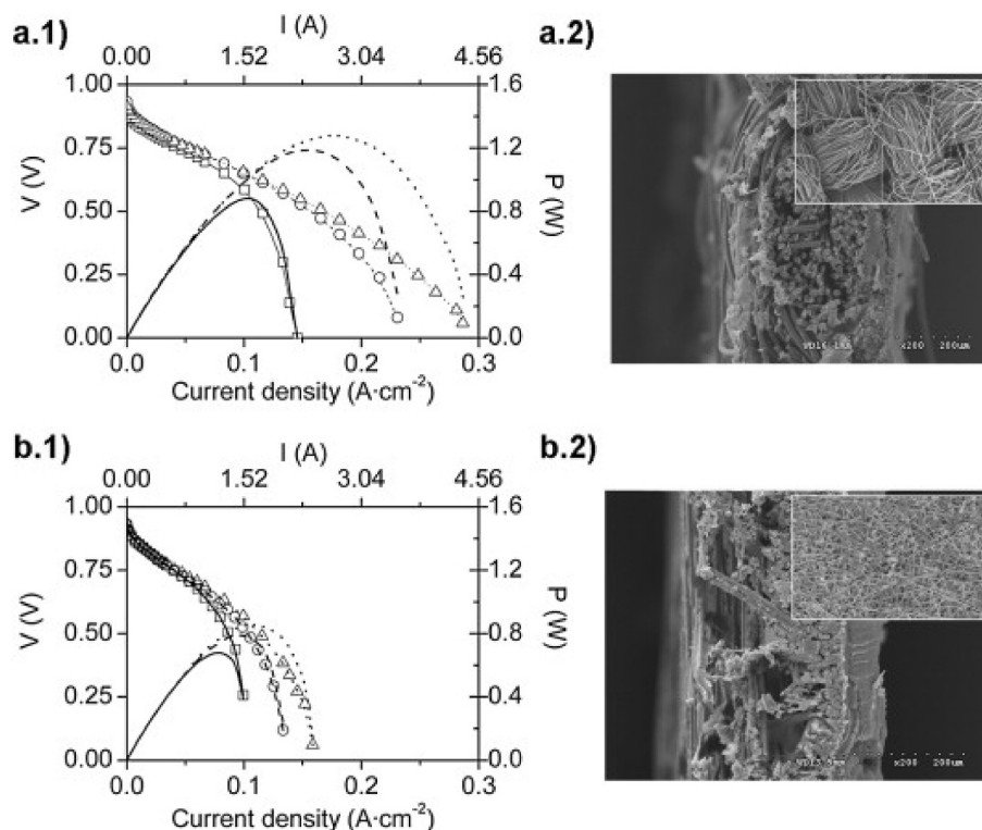
Fig. 9. Polarisation curves of the air-breathing PEFC with: a) woven GDL; b) non-woven GDL and with fan-driven air with maximum power (●●Δ●●), 18% of fan's maximum power (○●○), and natural convection (□□□). Reprinted with permission from Elsevier [83].
