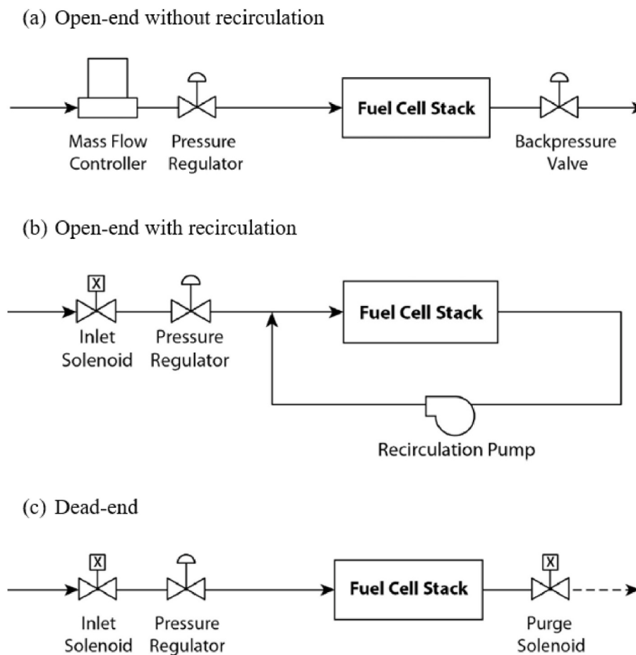
Fig. 13. Schematics of hydrogen supply modes: (a) open-end without recirculation, (b) open-end with recirculation and (c) dead-end. Reproduced from Ref. [118] with permission from Elsevier.
