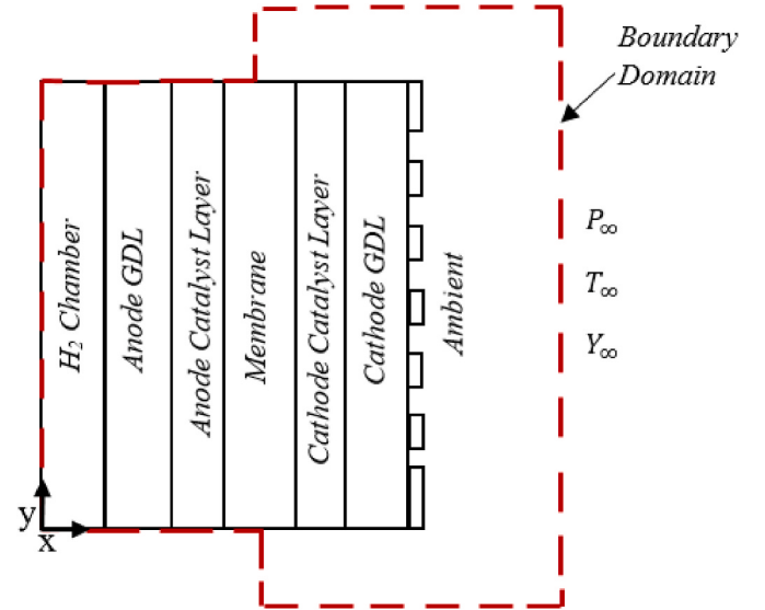
Fig. 2. A cross-section schematic of an air-breathing PEFC showing the boundary domain.
