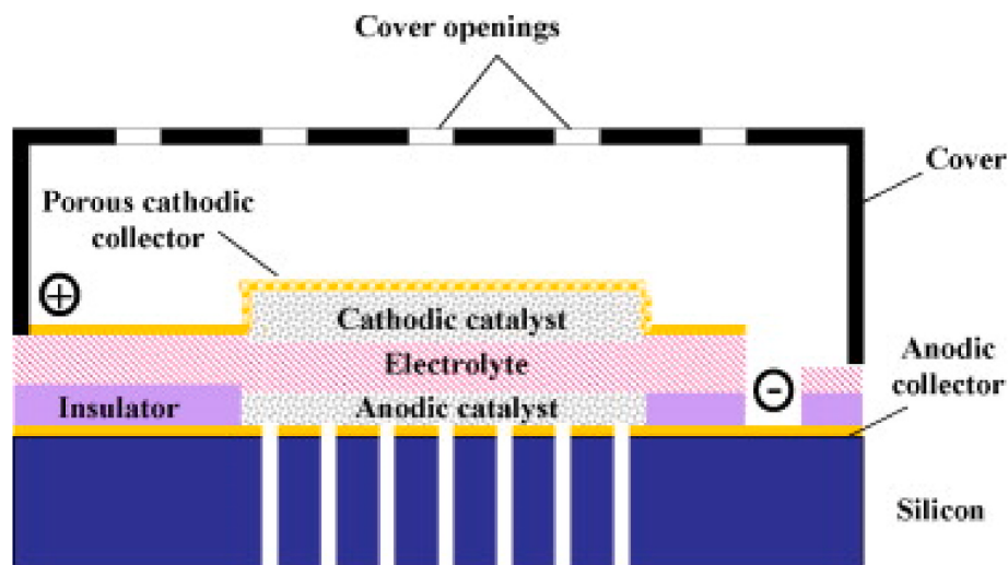
Fig. 7. A schematic of the cross-section of the air-breathing PEMFC equipped with the perforated cover. Reprinted with permission from Elsevier [73].
