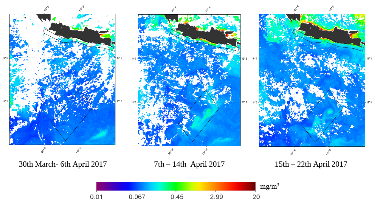
Figure 4. The 8-day composite data of chlorophyll-a variability in A1 and A2 region from 30 March – 22 April 2017.
