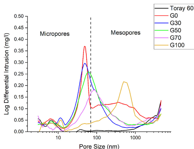
Fig. 3 – Pore size distributions of the microporous layer of the GDLs. The size of micropores is conventionally less than 70\text{ nm} and the size of the mesopores is between 70 and 5000\text{ nm} .
