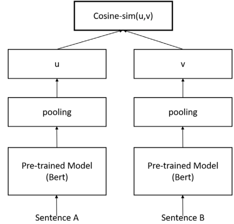
Fig. 2. The structure of calculating the sentence similarity uses Sentence BERT representations with cosine similarity. u and v are sentence embeddings. Note that the pre-trained models are fixed, and the process has no parameter update.
