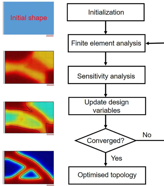
Figure 3. Flow chart of the topology optimisation procedure [35,47].
