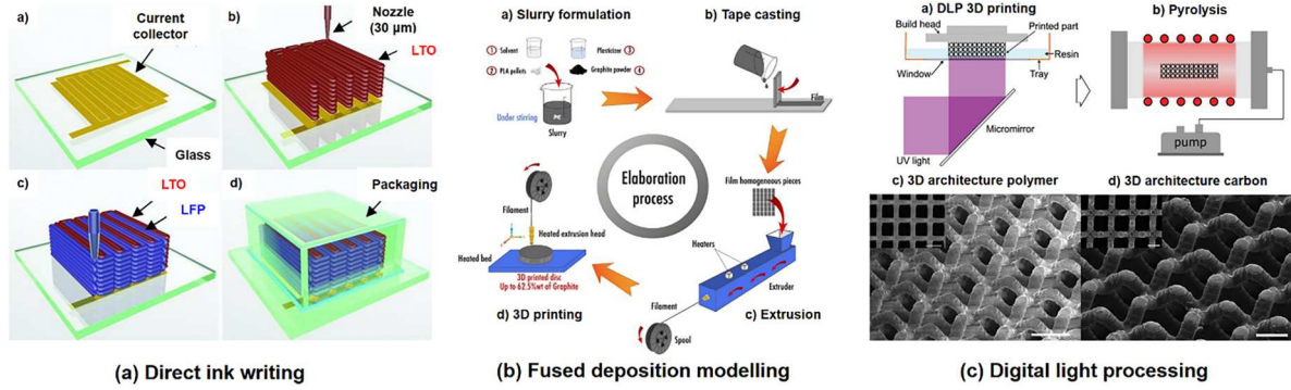
Figure 5. Additive manufacturing techniques for lithium-ion battery manufacturing: (a) Direct ink writing (DIW) [74] (b) Fused deposition modelling (FDM) [80] (c) Digital light processing (DLP) [81].
