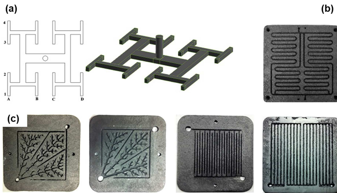
Figure 8. Fuel cell bipolar plate fabrication and design: (a) Constructal flow distributor [127] (b) Graphite bipolar plate with serpentine flow field [125] (c) Bio-inspired design and conventional interdigitated design [129].
