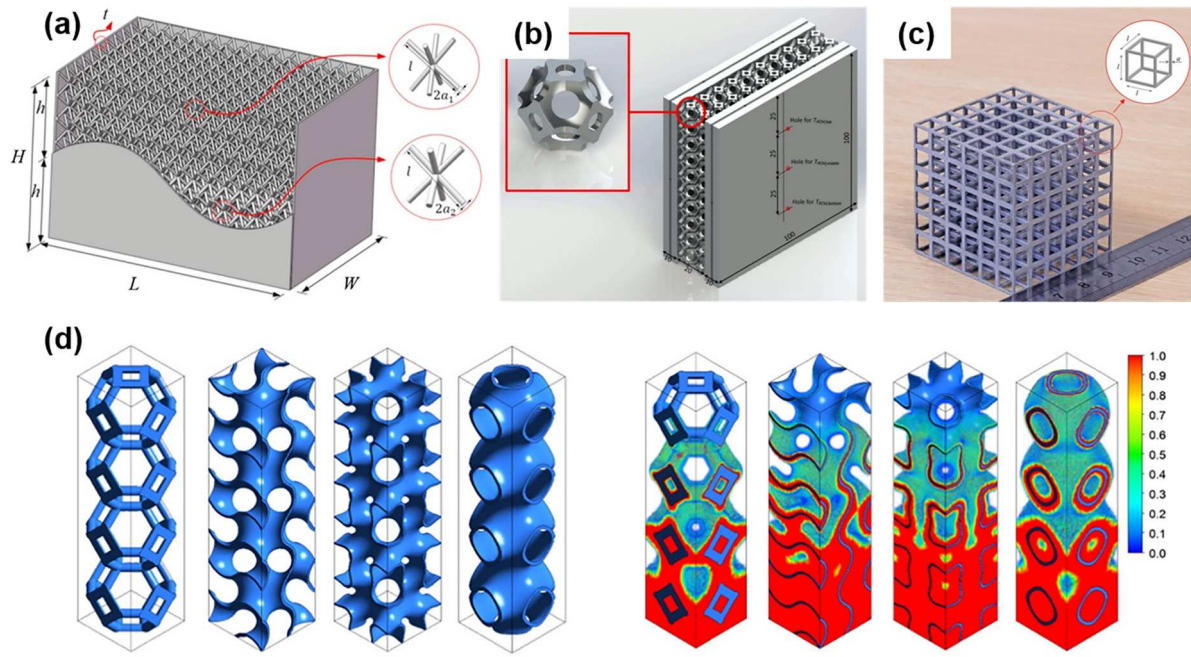
Figure 12. Impregnation of additive manufactured lattice structures: (a) Graded cellular design as thermal conductivity enhancer [26] (b) Periodic body-centred cubic cellular structures [27] (c) Periodic simple cubic cellular structures [28] (d) TPMS metal foam structures [29].
