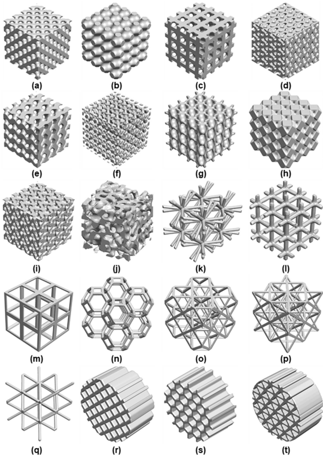
Figure 1. Various lattice structure types used for energy device: (a) TPMS Schwarz-D (b) TPMS Schwarz-P (c) TPMS Secondary I-WP (d) TPMS SplitP (e) TPMS Gyroid (f) TPMS Lidinoid (g) TPMS Neovius (h) TPMS Primary I-WP (i) TPMS FischerKoch (j) Stochastic structure (k) Hex truss (l) Face centre struts (m) Edge struts (n) Kelvin cell (o) Octagon struts (p) Face diagonal struts (q) Corner diagonal struts (r) Diamond (s) Hexagon (t) Triangle.
