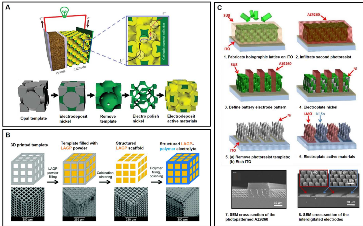
Figure 6. Fabrication of 3D structured lithium-ion batteries: (a) Illustration of a battery containing a bicontinuous cathode, and the electrode fabrication process [19] (b) 3D bicontinuous structured electrolyte [91] (c) 3D porous electrode fabricated by 3D holographic patterning technique [75].
