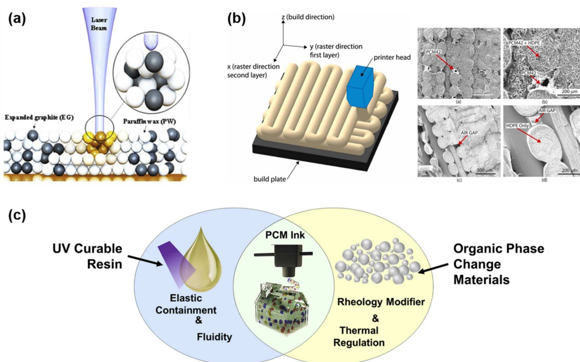
Figure 13. Demonstration of additive manufacturing of composite PCMs: (a) SLS process of paraffin wax/expanded graphite [168] (b) FFF process of composite PCMs, and illustration of printed samples e.g. PCM42/HDPE and HDPE [171] (c) DIW process of the polymer-PCM composites [173].
