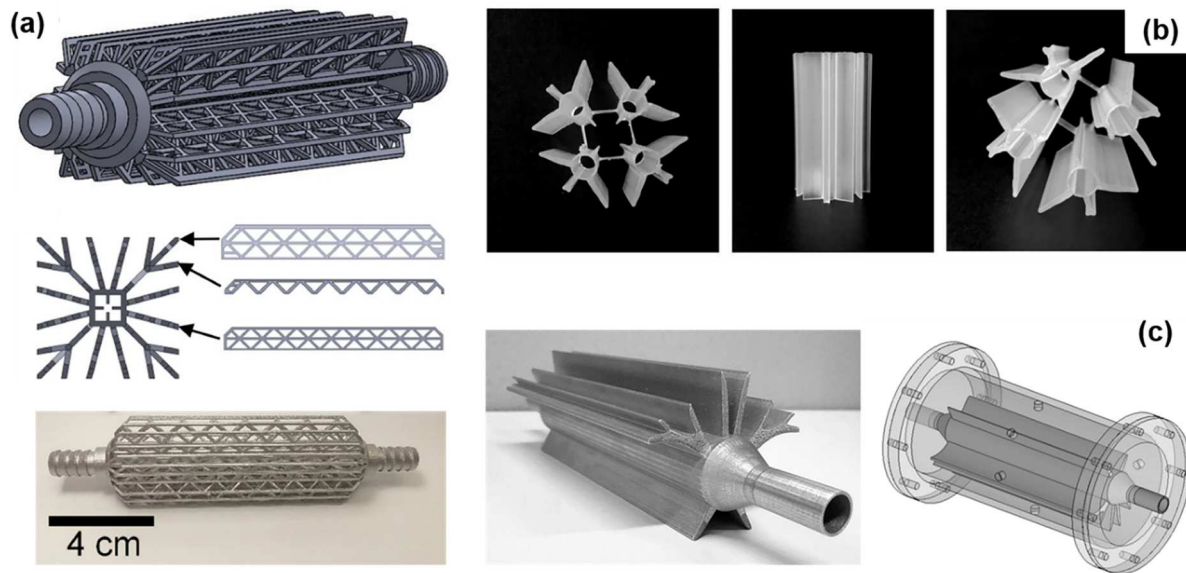
Figure 11. Additive manufactured fins and extended surfaces: (a) Additive manufactured device with external and internal fins to enhance heat transfer [71] (b) Additive manufactured multi-tube device with an optimised fin configuration [16] (c) Additive manufactured optimised fin configuration for melting performance enhancement [160].
