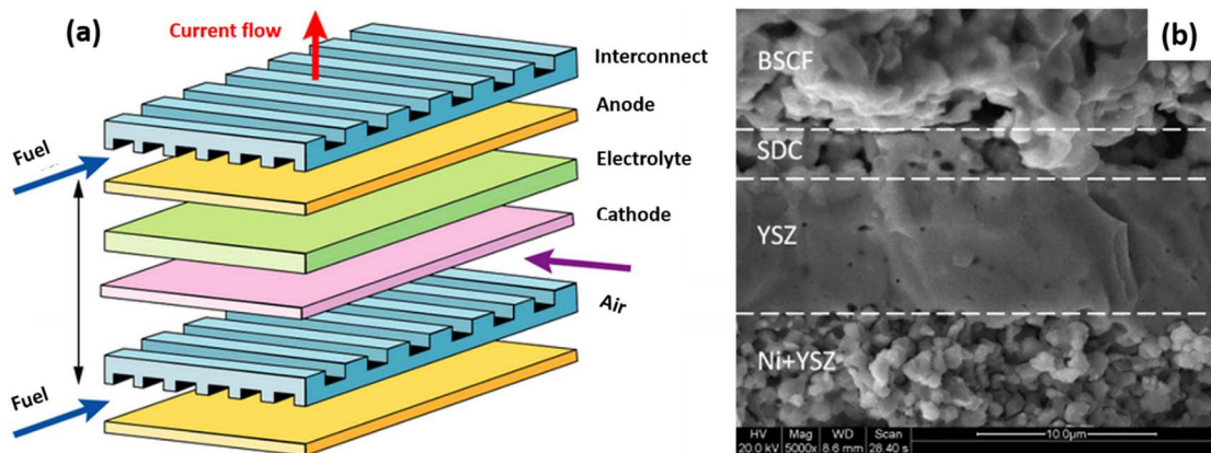
Figure 7. Illustration of a fuel cell stack: (a) Solid oxide fuel cell (b) Inkjet printing fabricated solid oxide fuel cell with a thin-film YSZ electrolyte, Ni+YSZ anode, SDC buffering layer, and BSCF cathode [118].
