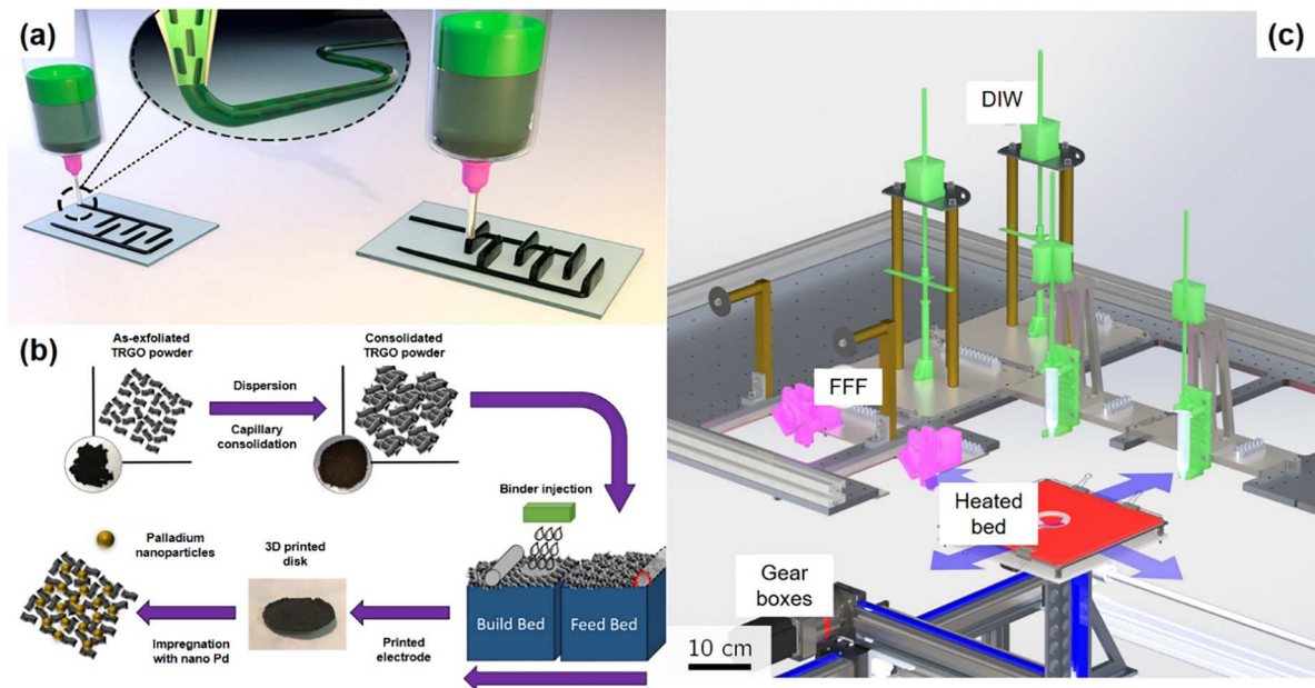
Figure 9. Additive manufacturing techniques for supercapacitor manufacturing: (a) Direct ink writing (DIW) of micro-supercapacitors (MSCs) with interdigital architectures [135] (b) Binder-jetting powder bed AM of thick graphene-based electrodes [136] (c) Hybrid additive manufacturing [137].
