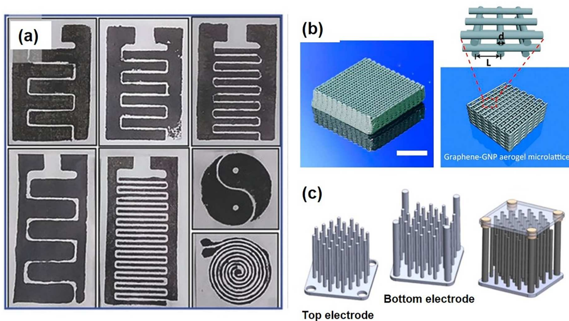
Figure 10. Additive manufacturing of supercapacitors: (a) Stamped MXene supercapacitors with various architectures [138] (b) Compressible graphene aerogel micro lattices fabricated by direct ink writing [140] (c) 3D interdigitated electrodes [141].
