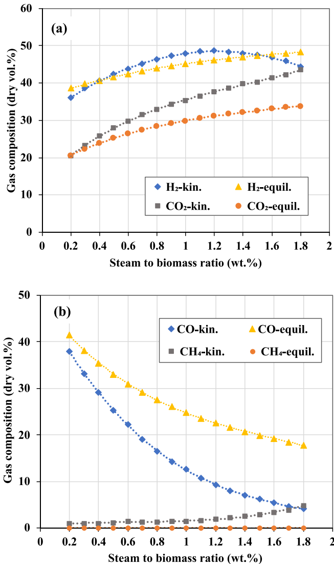
Fig. 10. Effect of SBR on the gas composition of the produced gas from the oxygen-based gasification process using the kinetic and the equilibrium models.
