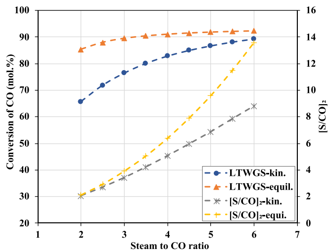
Fig. 14. Effect of the steam to CO ratio on the conversion of CO and on the intermediate S/CO prior to the LTWGSR under the kinetic and the equilibrium models.
