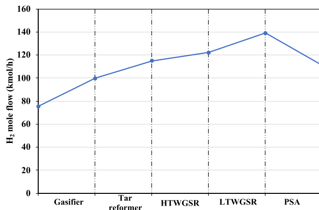
Fig. 15. Hydrogen buildup throughout the system components.
