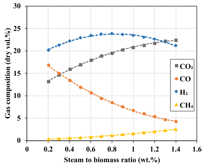
Fig. 8. Effect of SBR on the produced gas composition from the air-based gasification process.
