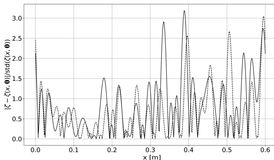
FIG. 8. Spatial variation of the relative error for the surface \zeta(x, \theta) of the mean of each parameter in the posterior (solid line), and the mean of the resulting surfaces \bar{\zeta}(x, \theta) (dashed line), against the true surface factored by the standard deviation of the true surface.
