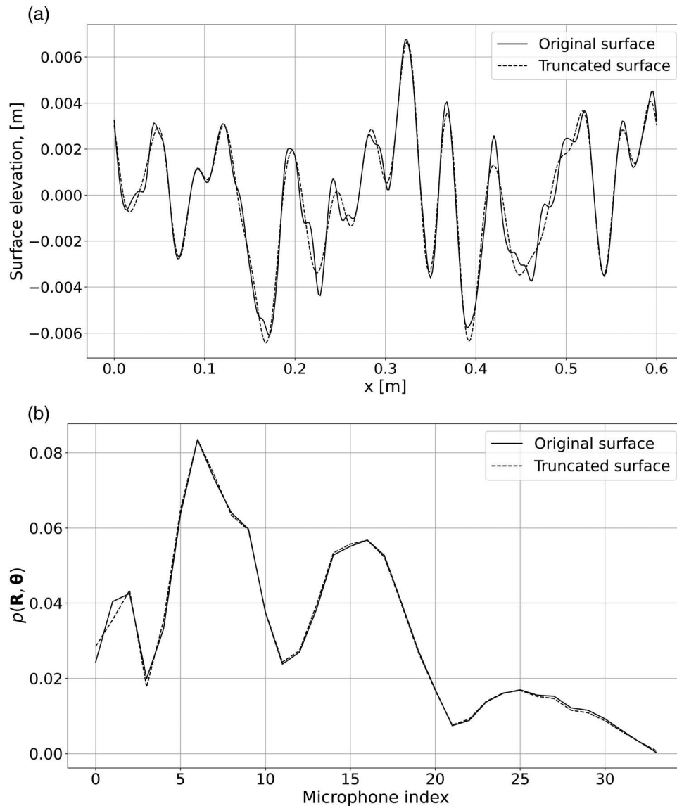
FIG. 6. Comparison of the second rough surface profile against the truncated sum of 20 sinusoidal waves for (a) the surface elevation, (b) the corresponding Kirchhoff approximation.
