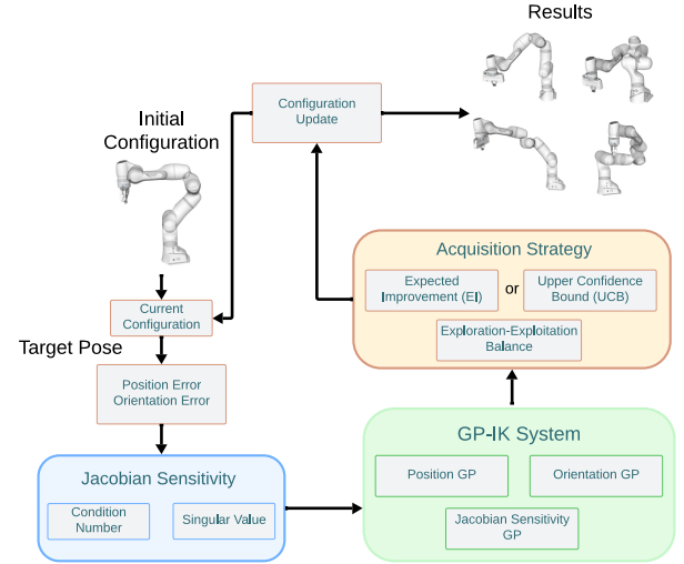
Fig. 1: The Jacobian-Guided GP- IK Framework that uses GP models to learn optimal movements, guided by an acquisition strategy that balances exploration and exploitation.
