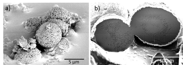
Figure 7. Calcium carbonate particles precipitated using a 0.2 μm ceramic membrane at a \text{CO}_2 flow rate of 0.1 L/min in the absence of applied shear showing (a) spherical vaterite particles composed of a “rod” like primary particles and a porous surface structure and (b) particles milled with a focused ion beam revealing a solid internal core and areas of inherent porosity.
