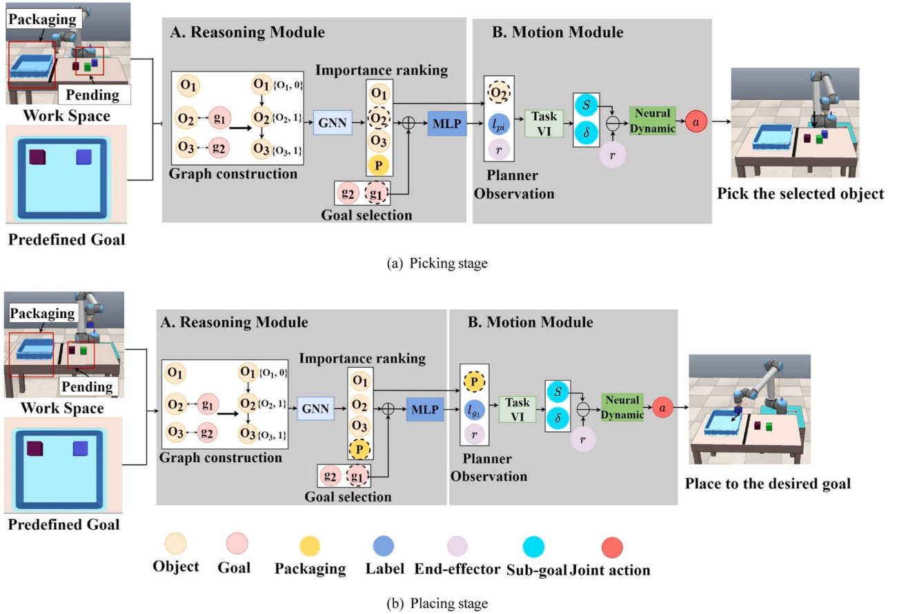
Fig. 2. Graphic representation of proposed framework at picking and placing stage. At picking stage, the reasoning module will always focus on the selected objects in the pending area while at the placing stage, it will always focus on the packaging box observations.
