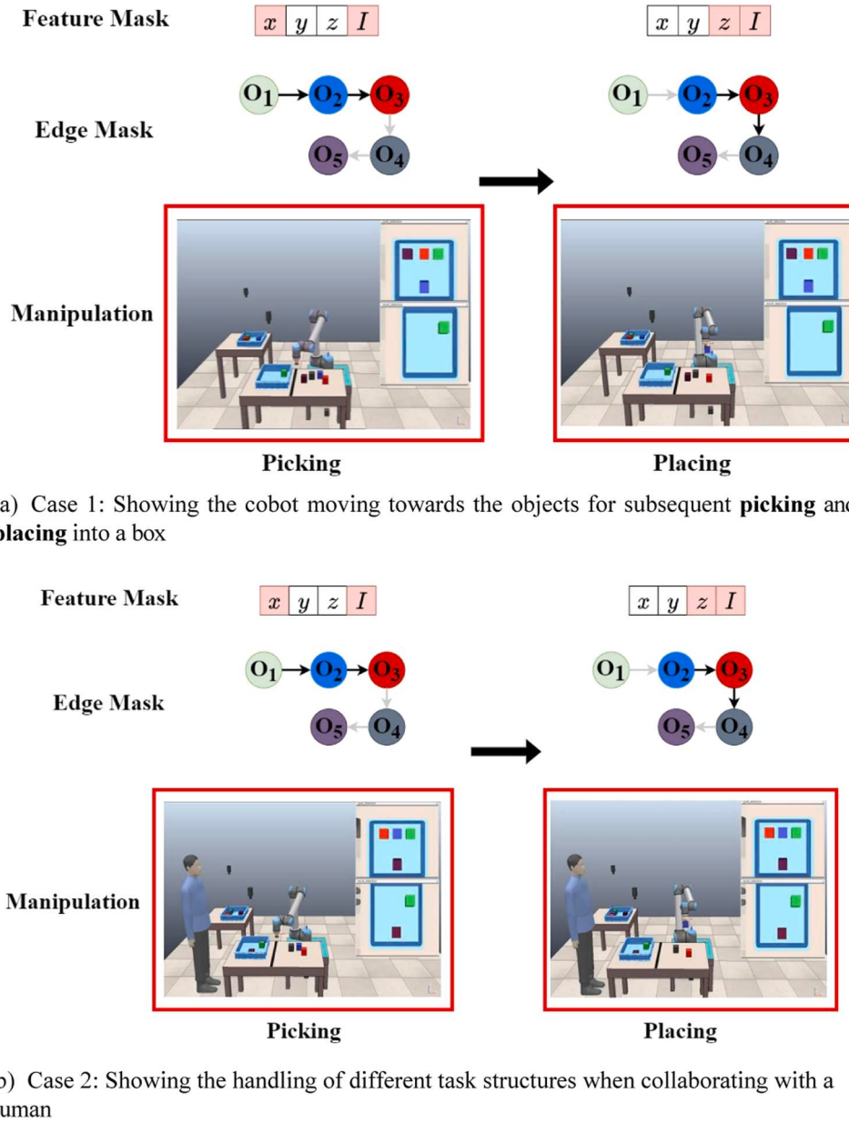
Fig. 10. We interpret the learnt reasoning module at picking and placing in two different cases. For each sub-figure above, the first row (Feature mask) describes the most important features and the second row (Edge mask) indicates the most important edges as solid lines. The third row describes the manipulation scenes from the simulation.
