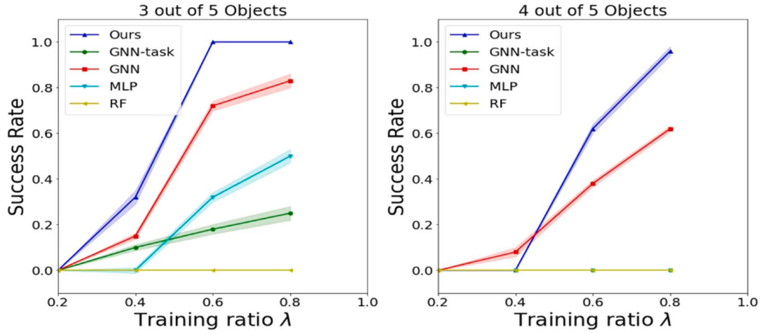
(a) Generalization study on handling unseen goal configurations in CASE 1
