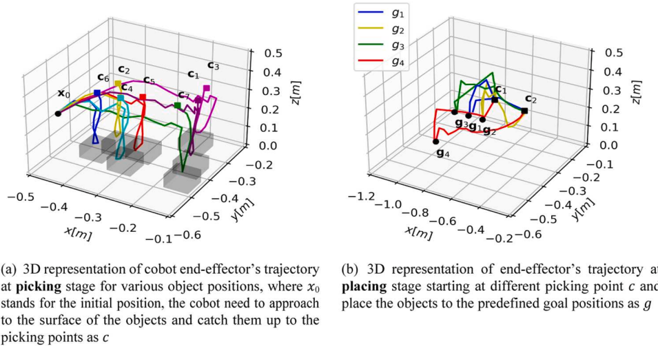
Fig. 13. The 3D reproduction trajectory from our motion module trained from 4 out 5 objects experiments.
