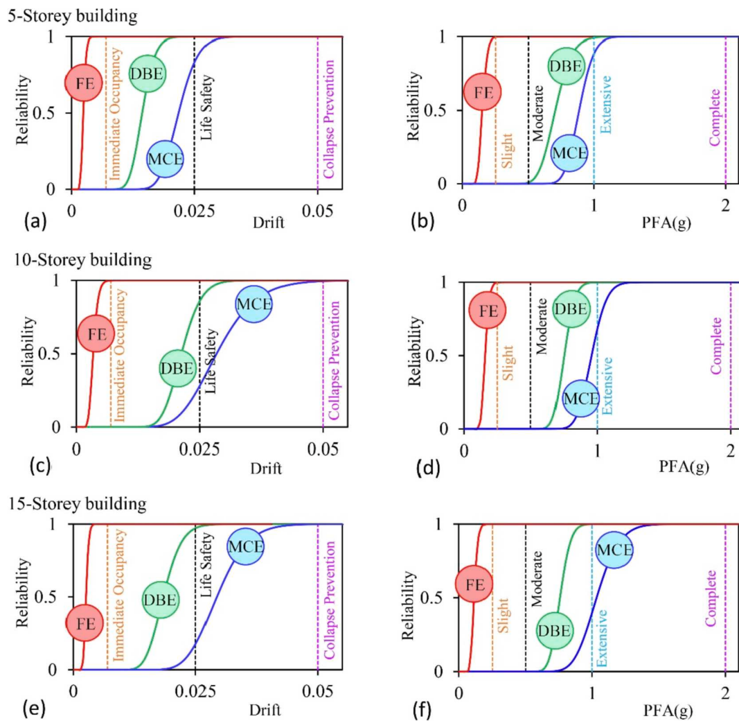
Fig. 6. Reliability curves obtained with the standard approach for the structural (a, c and e) and non-structural components (b, d and f), under different hazard levels and for limit states corresponding to different damage levels.
