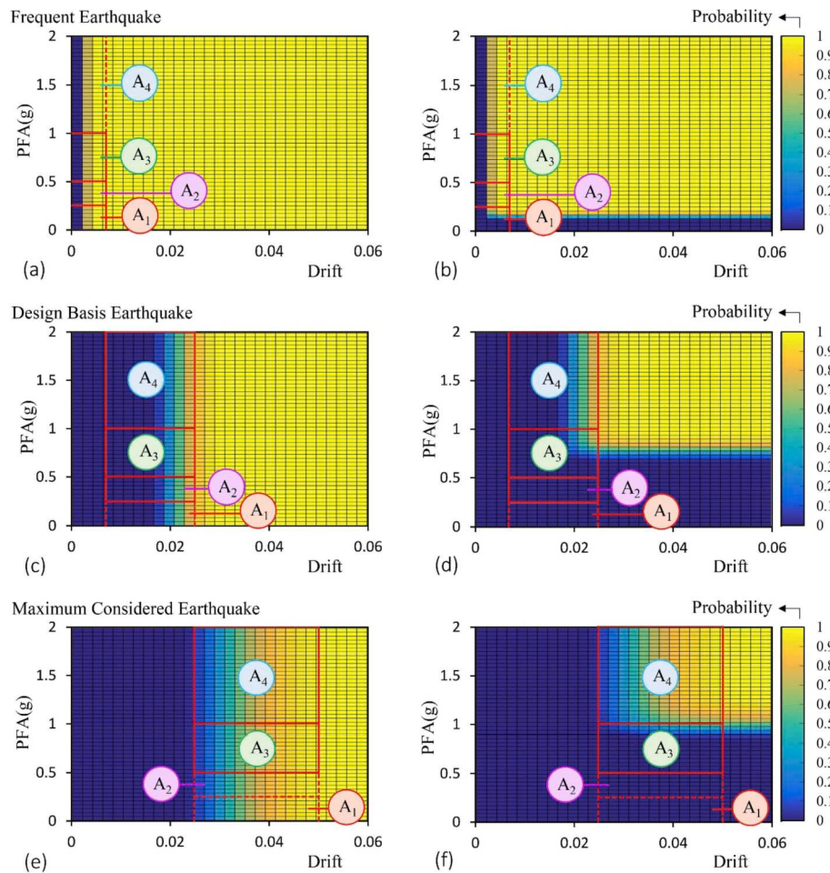
Fig. 19. Reliability levels of the 10-story structure, under: FE (a and b), DBE (c and d), and MCE (e and f). Results obtained by considering the structural components only (a, c and e), or both the structural and non-structural components (b, d and f).
