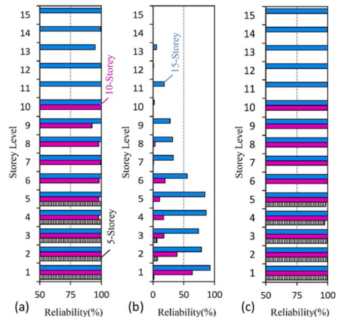
Fig. 9. Design basis earthquake, story-wise reliability corresponding to: (a) LS performance level for the structural components; (b) Moderate damage level for the non-structural components; (c) Extensive damage level for the non-structural components.
