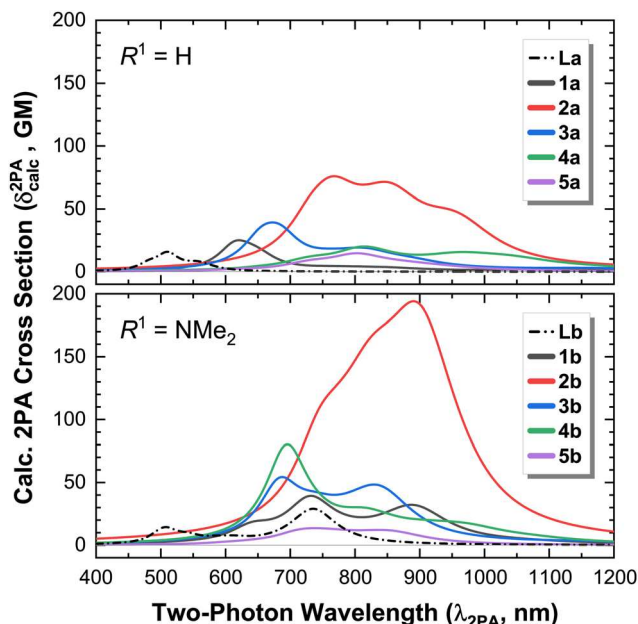
Fig. 7 Calculated two-photon absorption (2PA) spectra of complexes ( 1–5 ) a , and ligand La ( R^1 = \text{H} , top); and complexes ( 1–5 ) b and ligand Lb ( R^1 = \text{NMe}_2 , bottom). The vertical scale of both figures is identical to facilitate comparison.
