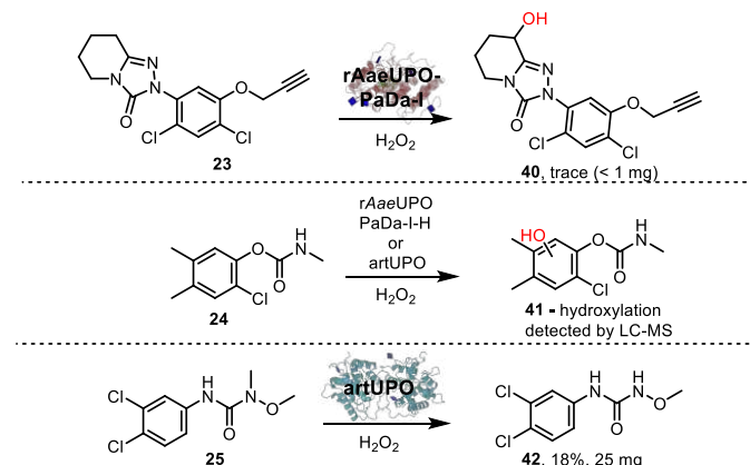
Scheme 5. UPO transformations of halogenated aromatics.
