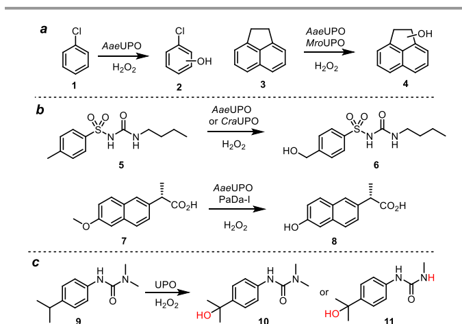
Scheme 1. UPOs as broad-spectrum oxidants in compound oxygenation: a: as applied to environmental pollutants; b: as applied to pharmaceuticals; c: as applied to agrochemicals.
