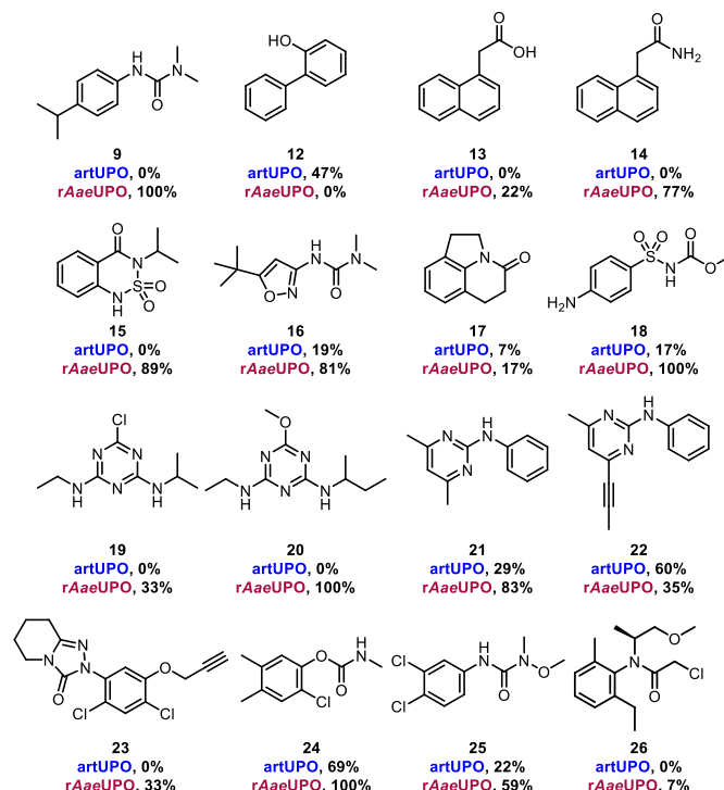
Figure 1. Summary of substrates undergoing conversion (%) in an LC-MS screen of agrochemical oxygenation by rAaeUPO-PaDa-I-H ('rAaeUPO') and artUPO
