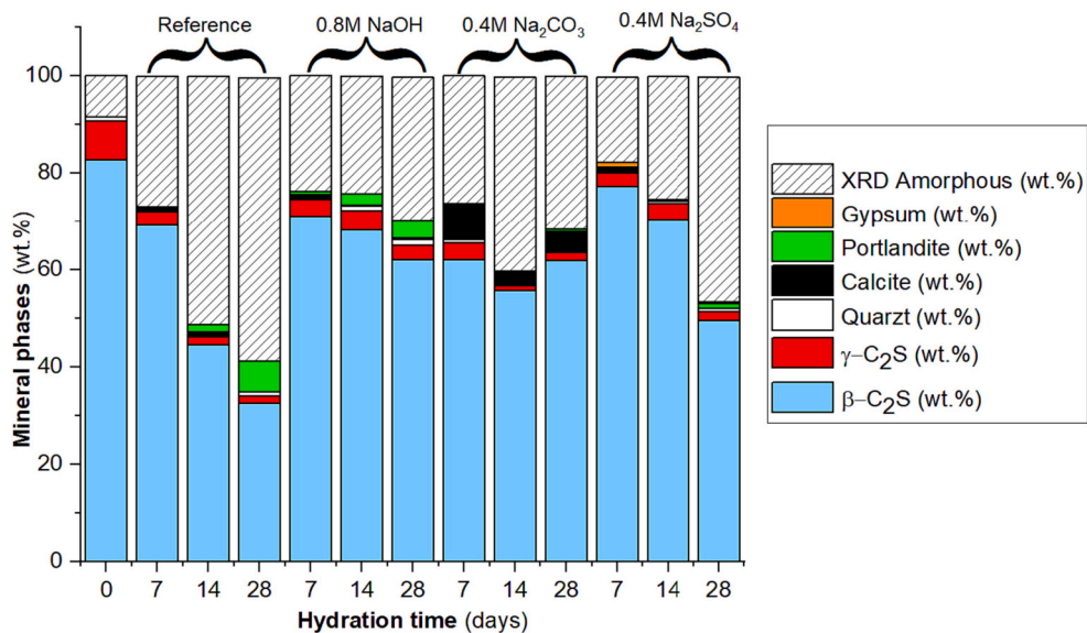
Fig. 4. Quantitative X-ray diffraction (QXRD) of chemically activated \beta -C 2 S at curing ages of 7, 14, and 28 days with a 1.6 w/s ratio.
