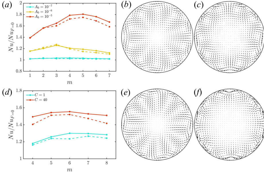
Figure 17: Optimisation at larger parameters. Top row: C = 16 , Re = 3000 , A_0 in key to (a), O_{F5} at A_0 = 10^{-5} for steady and unsteady flow in (b) and (c). Bottom row: Re = 5000 , A_0 = 10^{-5} , C in key to (d), O_{F6} at C = 1 for steady and unsteady flow in (e) and (f). In (a,d), solid is for the turbulent state, and dashed line indicates a force optimised with a steady state. The largest arrow has magnitude 1.4 \times 10^{-3} in (b), 1.9 \times 10^{-3} in (c), 1.7 \times 10^{-3} in (e) and 2.4 \times 10^{-3} in (f).
