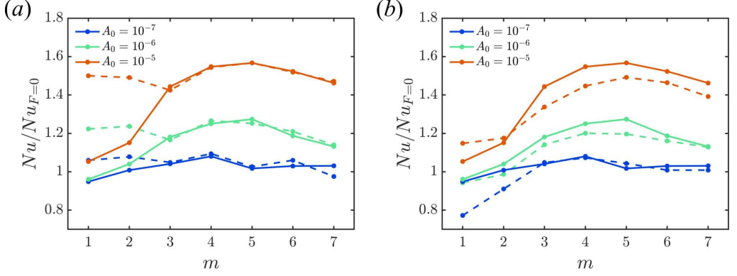
Figure 13: Normalised Nusselt numbers for flows at C = 1 , Re = 3000 subject to optimal forces in the full and reduced rotational symmetries. (a) Comparison between O_{Fm} (solid lines) and O_m (dashed lines). (b) Comparison between O_{Fm} optimised for shear turbulence (solid line) and a steady two-dimensional laminar state (dashed line).
