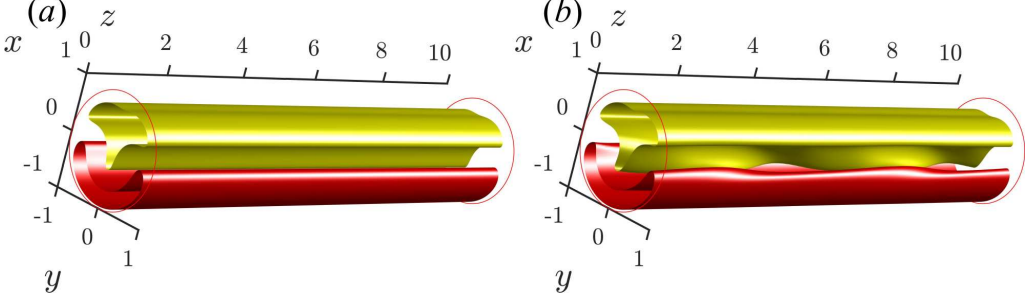
Figure 8: Isosurfaces of streamwise velocity for (a) the streamwise-independent state at t = 500 and (b) the travelling wave solution at t = 1500 , for flow forced by O_{F1} with A_0 = 6 \times 10^{-7} . Red/yellow are at 20% of the min/max streamwise velocity.
