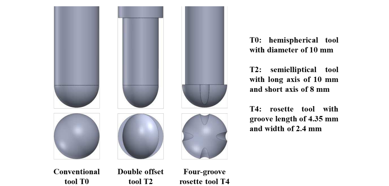
Fig. 1. Tool design: conventional tool T0, double offset tool T2 and four-groove tool T4.
