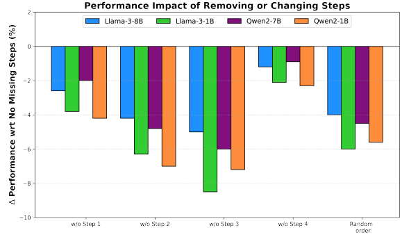
Figure 2: Performance differences ( \Delta ) for each tuned model. We analyse the impact of each component on tuning by eliminating (w/o) or random shuffling the four QuaSAR steps.
