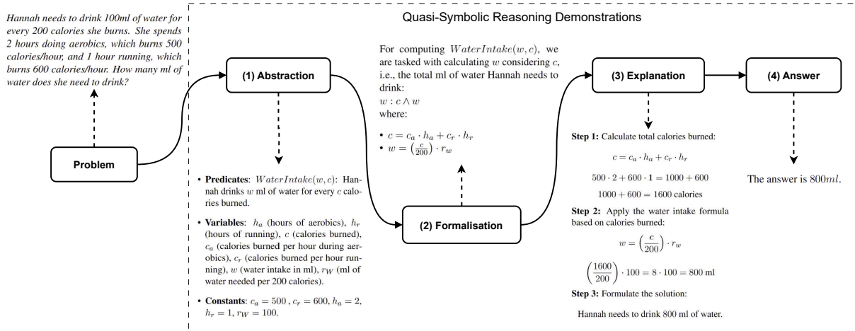
Figure 1: QuaSAR elicits quasi-symbolic abstractions in LLMs via the following steps: (i) Abstraction , where the problem is analysed and abstracted in terms of relevant symbolic predicates, variables, and constants; (ii) Formalisation , where the original problem is reformulated using a mixture of symbolic expressions and natural language; (iii) Explanation , where the necessary steps to compute the solution are formulated via quasi-symbolic reasoning chains; and (iv) Answering , where a final solution is generated. We use QuaSAR as an in-context learning strategy and for constructing reasoning demonstrations for smaller LLMs.
