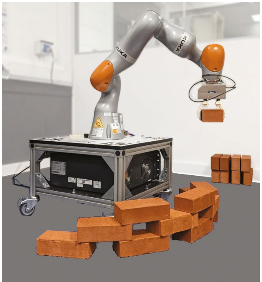
Figure 3: Brick wall construction with end pose data transferred from parametric CAD design.
