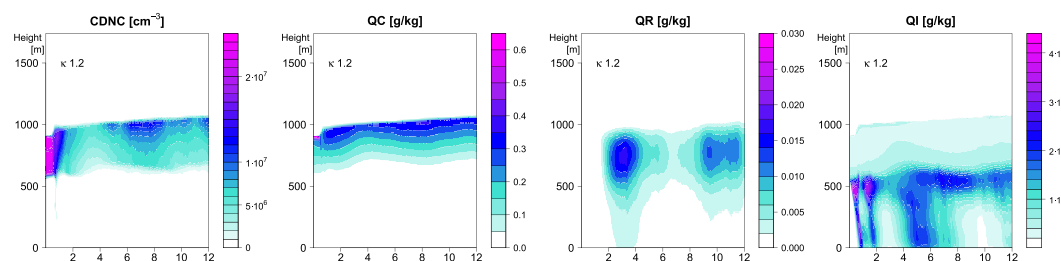
Figure 9. Evolution of horizontally averaged cloud microphysical parameters (cloud droplet number concentration (CDNC), cloud water (QC), rain water (QR), and cloud ice (QI)) simulated for hygroscopic aerosols with a maximum \kappa of 1.2. The simulation is from the set Aitken_30.
