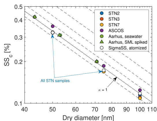
Figure 4. (left) Critical supersaturation as a function of dry mobility diameter in of four SML samples. For comparison inorganic sea salt and results from Rasmussen et al. (2017) are added. (right) Map of sampling locations.
