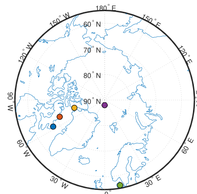
Figure 4. (left) Critical supersaturation as a function of dry mobility diameter in of four SML samples. For comparison inorganic sea salt and results from Rasmussen et al. (2017) are added. (right) Map of sampling locations.
