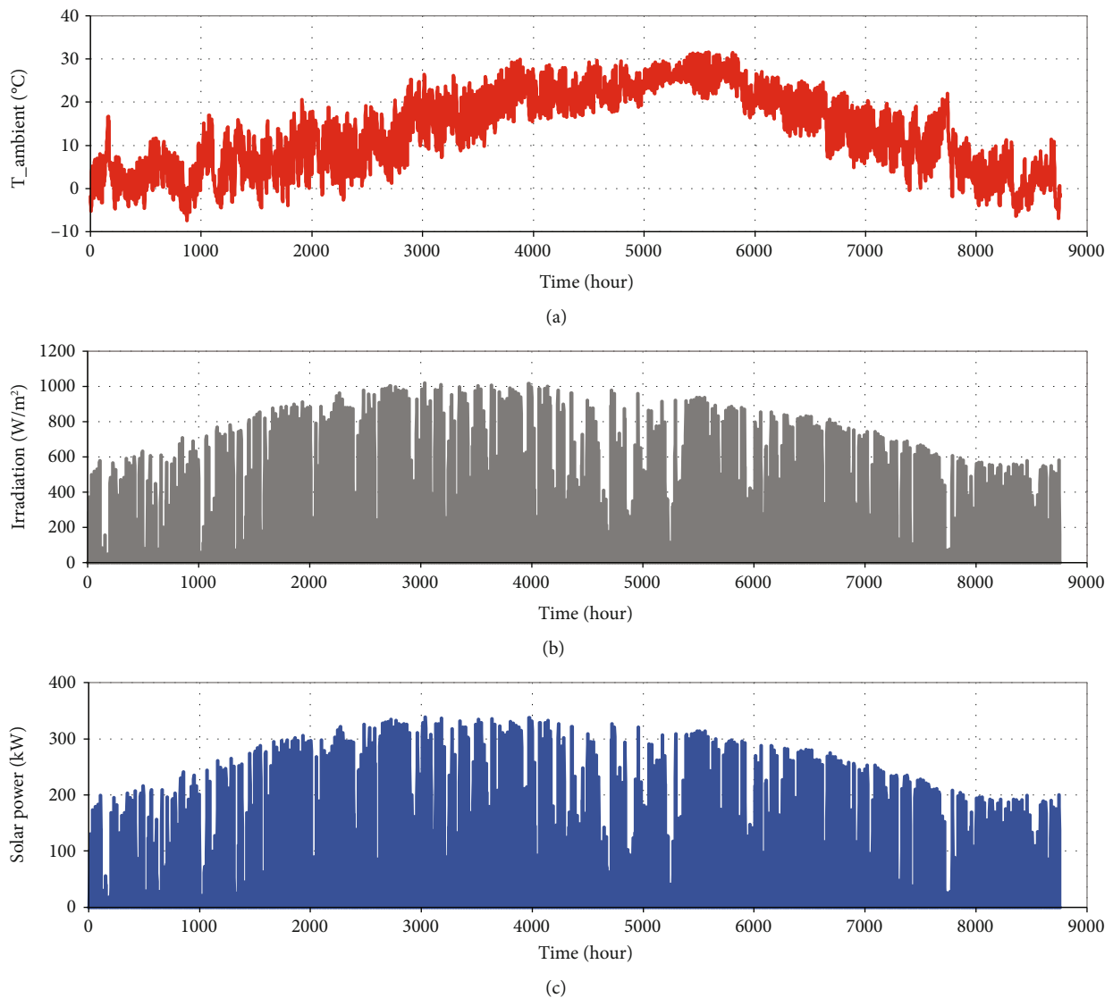
FIGURE 6: The ambient temperature (a), the solar irradiation (b), and the PV power generation (c) across one year at the smart farm location.
