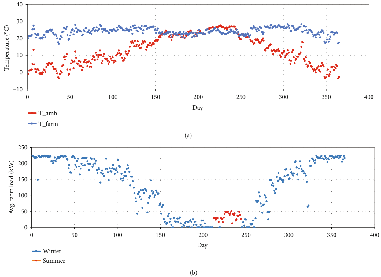
FIGURE 9: The predicted farm temperature (a) and the average farm heat load (b) on a daily basis over one year; red dots in graph (b) refer to cooling load.
