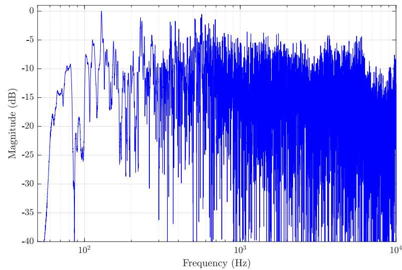
Figure 17. Frequency spectrum of the the impulse response obtained within the Triforium Level Library (FFT size = 4096 samples).
