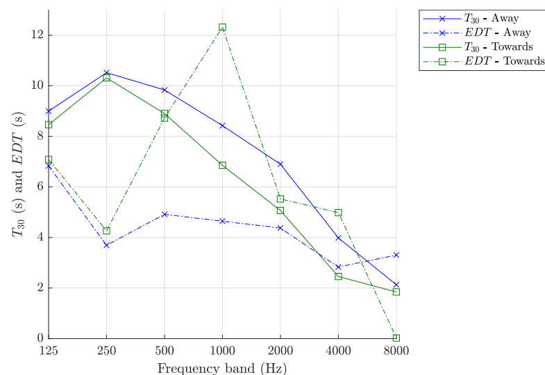
Figure 11. T_{30} (s) and EDT (s) results for two source-receiver configurations at the Whispering Gallery: 'Away' for when the source is oriented away from the receiver to be parallel to the wall; 'Towards' for when the source is oriented to directly face towards the receiver.
