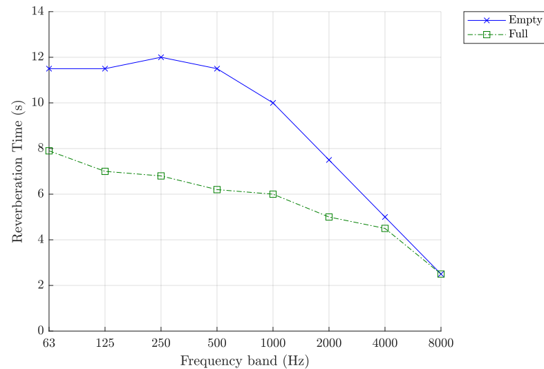
Figure 3. Reverberation time measurements for the nave (Empty and Full) of St Paul's, as obtained from Parkin and Taylor's work in 1952. The values presented here are based on the numerical data presented in relevant charts in [30].
