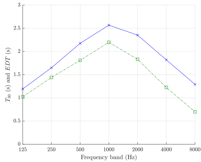
Figure 15. T_{30} (s) and EDT (s) obtained from the impulse response measured within the Triforium Level Library.
