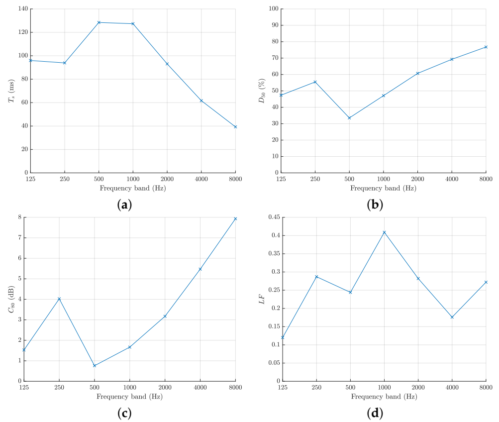
Figure 16. Results for (a) T_s , (b) D_{50} , (c) C_{80} and (d) LF obtained from the impulse response measured within the Triforium Level Library.
