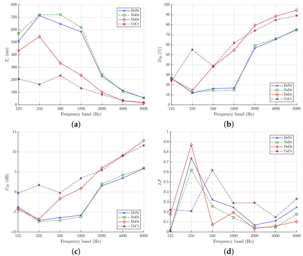
Figure 8. Results for the four source-receiver configurations obtained from the Cathedral floor for (a) T_s , (b) D_{50} , (c) C_{80} and (d) LF .
