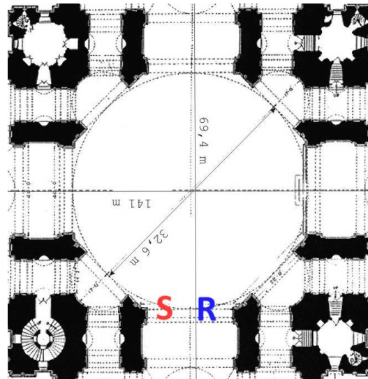
Figure 10. Floor plan of the Whispering Gallery of St Paul's Cathedral showing the source and receiver positions used for the measurements. Adapted file from Wikimedia Commons under the CC BY-SA 4.0 licence [32].
