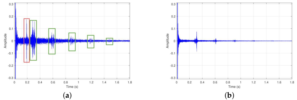
Figure 13. Time domain impulse responses for two source-receiver configurations at the Whispering Gallery: (a) ‘Away’ for when the source is oriented away from the receiver to be parallel to the wall; (b) ‘Towards’ for when the source is oriented to directly face towards the receiver.
