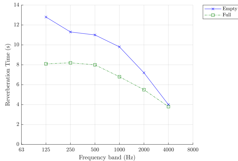
Figure 5. Reverberation time measurements for the nave (empty and full) of St Paul’s, as obtained by Lewers and Anderson in 1984. The values presented here are based on the numerical data presented in relevant charts in [2].
