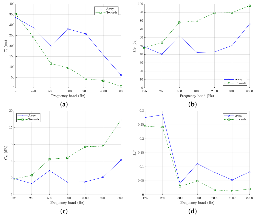
Figure 12. Results for (a) T_s , (b) D_{50} , (c) C_{80} and (d) LF for two source-receiver configurations at the Whispering Gallery; ‘Away’ for when the source is oriented away from the receiver to be parallel to the wall; ‘Towards’ for when the source is oriented to directly face towards the receiver.
