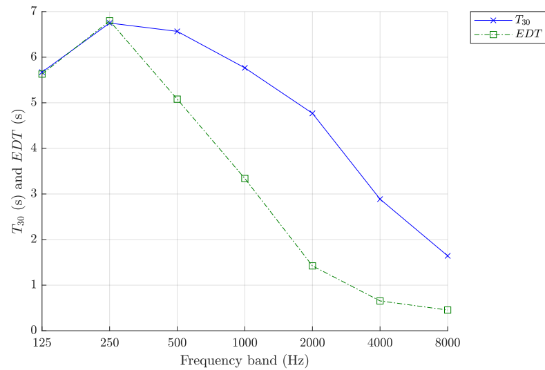
Figure 19. T_{30} (s) and EDT (s) obtained from the impulse response measured in the Geometric Staircase.
