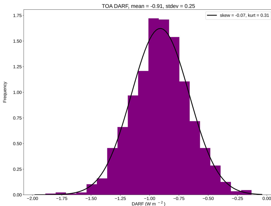
Figure 5. Example histogram generated by 500 samples of global annual mean direct aerosol radiative forcing (DARF) at the top of the atmosphere (TOA), in W m -2 , for \sigma_{\text{AOD}} = 0.03 , \sigma_{\omega_0} = 0.02 , and \sigma_g = 0.02 .
